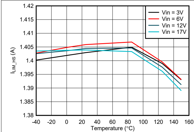
图 7-13. High-Side I_{LIM} vs Temperature
