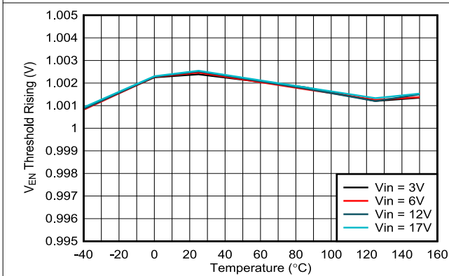
图 7-17. Precision Enable Threshold vs Temperature
