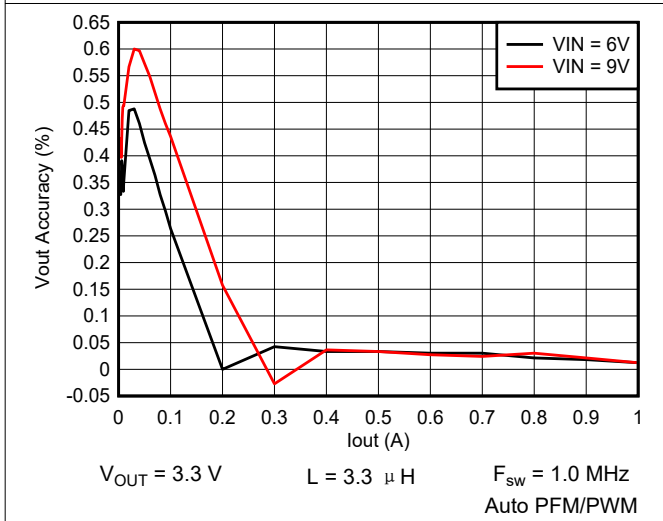
图 9-24. Output Voltage vs Output Current
