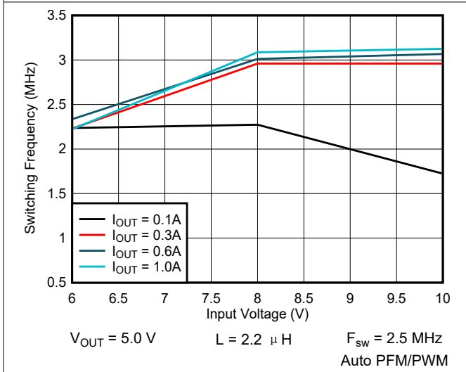
图 9-4. Switching Frequency vs Input Voltage
