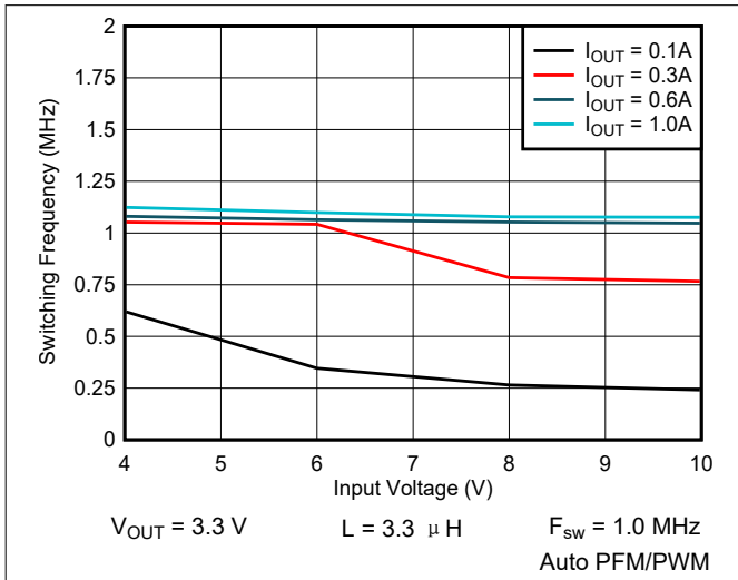
图 9-22. Switching Frequency vs Input Voltage
