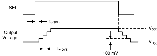
图 6-10. Dynamic Voltage Scaling with High Load
