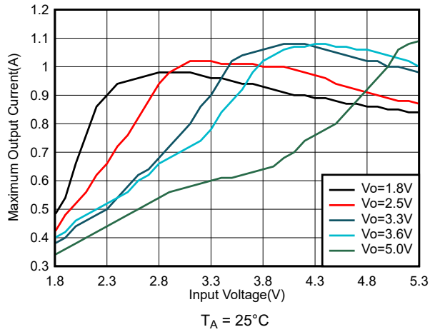
图 7-5. Typical Output Current Capability vs Input Voltage
