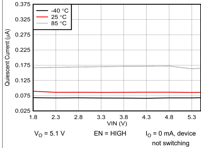
图 5-2. Quiescent Current into VOUT vs Input Voltage
