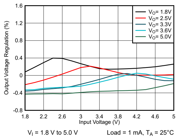
图 7-13. Line Regulation
