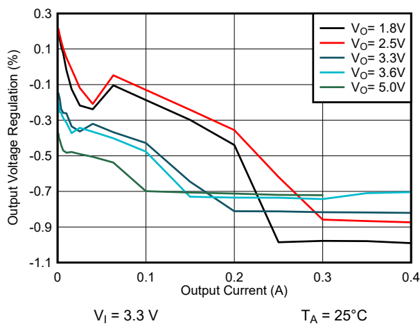
图 7-12. Load Regulation
