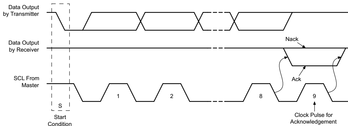
Figure 16. I 2 C Acknowledgment
