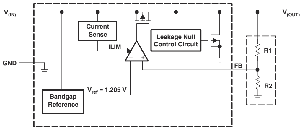
图 7-1. Functional Block Diagram—Adjustable Version
