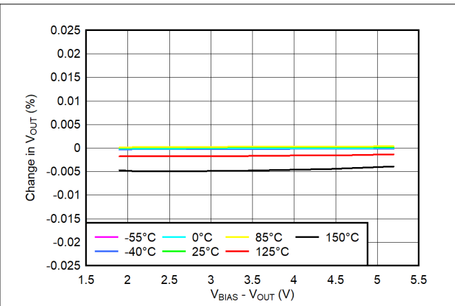
图 6-23. V BIAS Line Regulation
