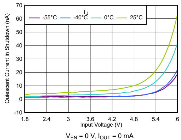
图 6-12. Shutdown Current vs V_{IN}
