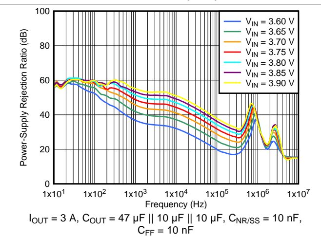
图 6. PSRR vs Frequency and V_{IN} for V_{OUT} = 3.3\text{ V}
