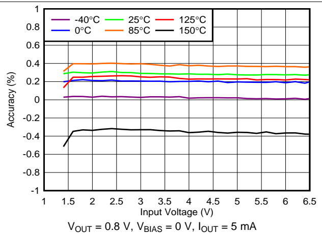
图 26. Line Regulation Without Bias
