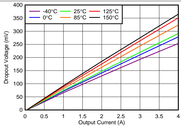
图 22. Dropout Voltage vs Output Current Without Bias
