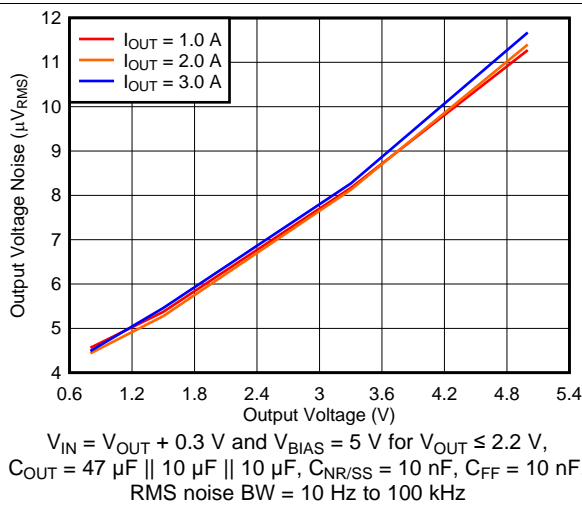
图 9. Output Voltage Noise vs Output Voltage
