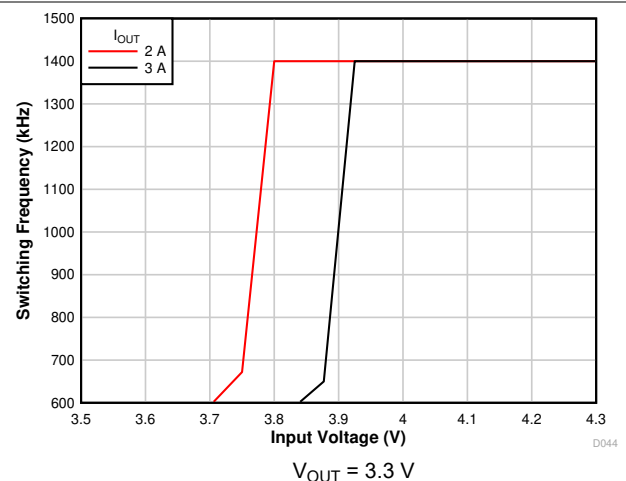
图 7-8. Frequency Foldback
