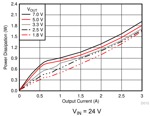
图 6-15. Power Dissipation versus Output Current
