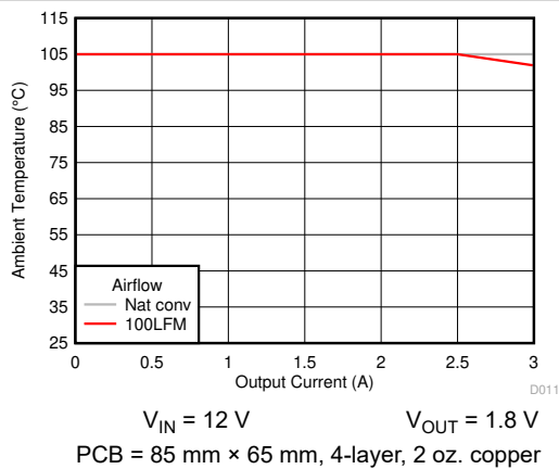
图 6-11. Safe Operating Area
