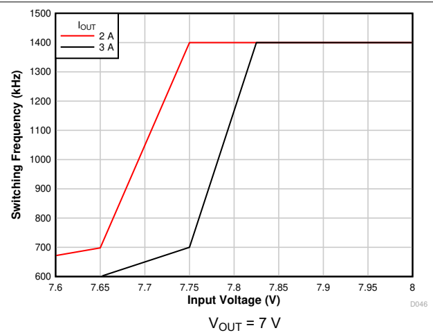
图 7-12. Frequency Foldback
