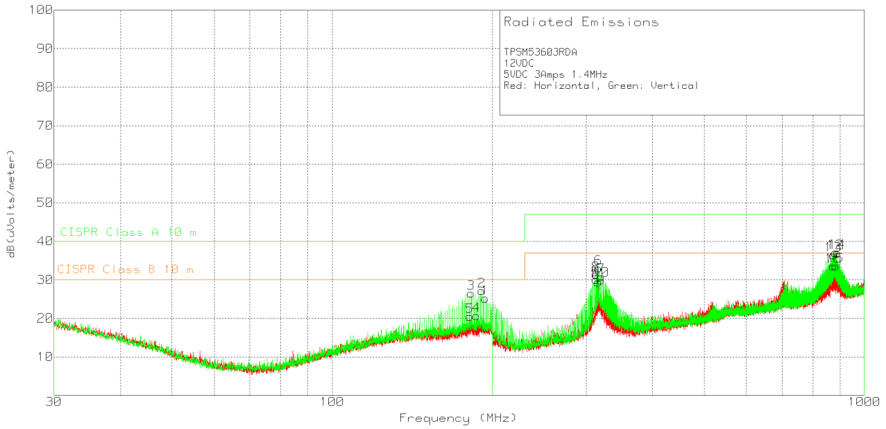
图 10-6. Radiated Emissions 12-V Input, 5-V Output, 3-A Load
