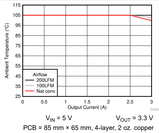
图 6-6. Safe Operating Area
