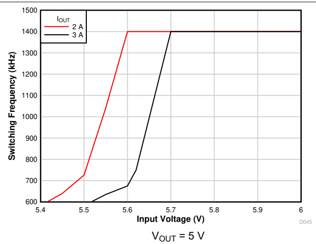
图 7-10. Frequency Foldback
