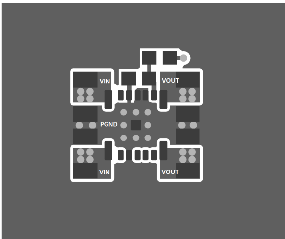
图 10-1. Typical Top-Layer Layout
