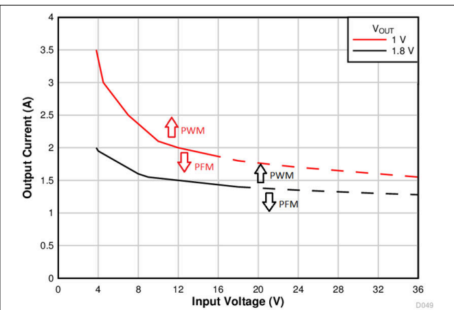
图 7-15. PFM/PWM Thresholds (1 V and 1.8 V)
