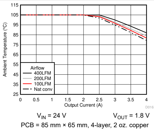
图 6-17. Safe Operating Area
