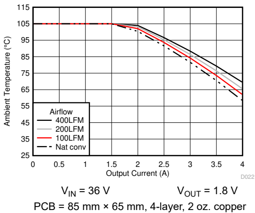
图 6-23. Safe Operating Area
