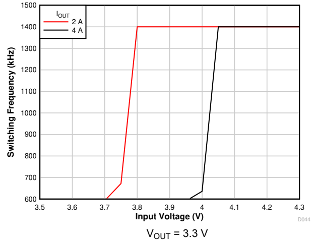
图 7-8. Frequency Foldback
