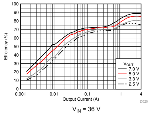
图 6-20. Efficiency versus Output Current
