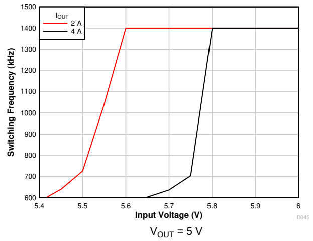
图 7-10. Frequency Foldback
