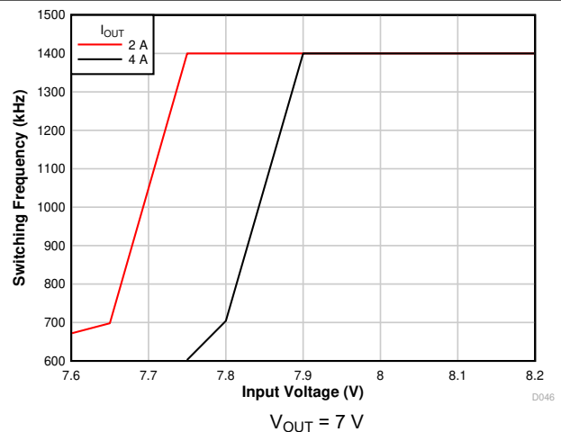
图 7-12. Frequency Foldback
