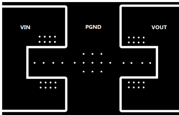
图 10-3. Typical Mid-Layer
