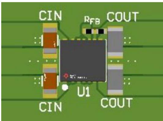
图 10-1. Typical Layout
