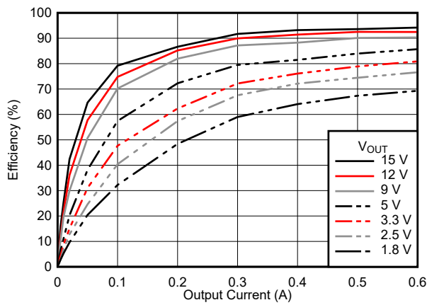
图 6-5. Efficiency
