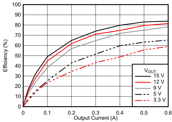
图 6-15. Efficiency
