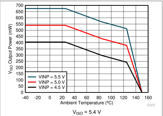
图 6-5. Maximum V_{ISO} Output Power vs. Temperature
