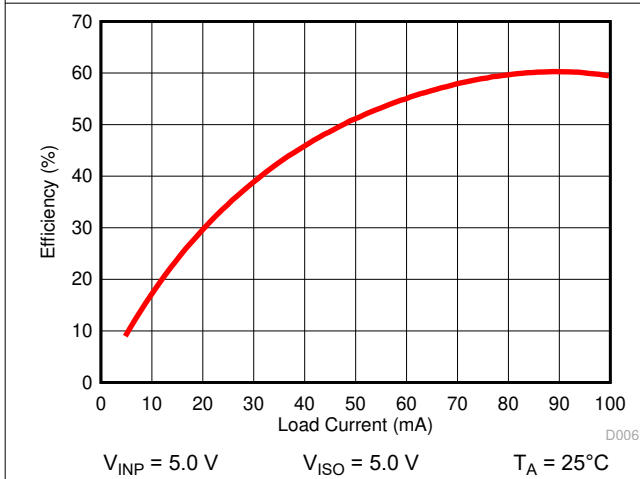
图 6-12. Power Supply Efficiency vs Load Current ( I_{ISO} )
