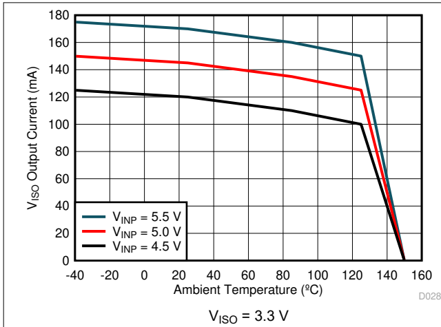
图 6-10. Maximum V_{ISO} Output Current vs. Temperature
