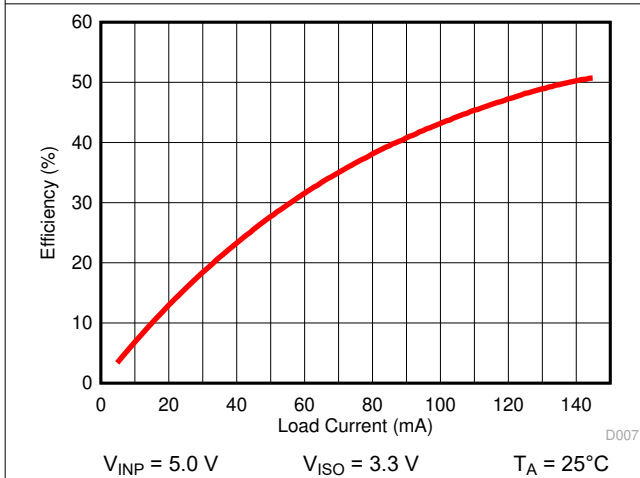
图 6-14. Power Supply Efficiency vs Load Current ( I_{ISO} )
