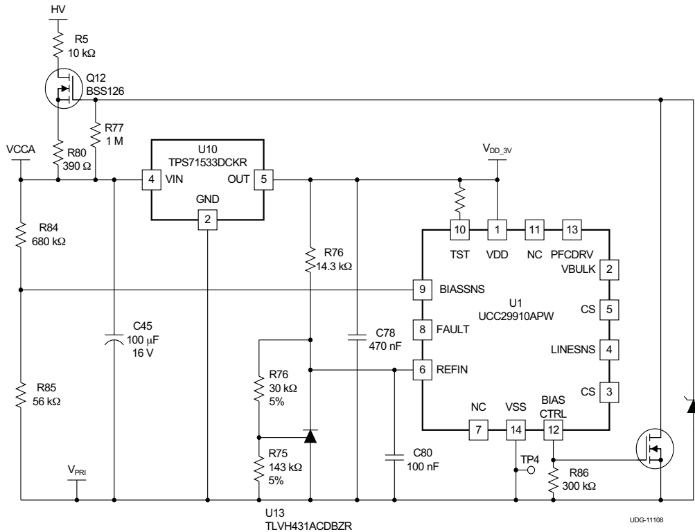
图 5. Simplified Schematic
