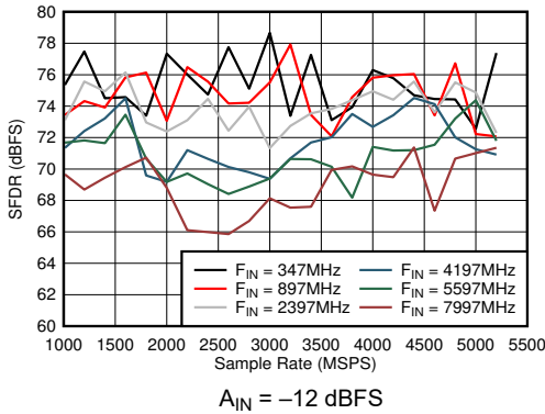
Figure 5-49. Dual Channel Mode: SFDR vs Sample Rate and Input Frequency
