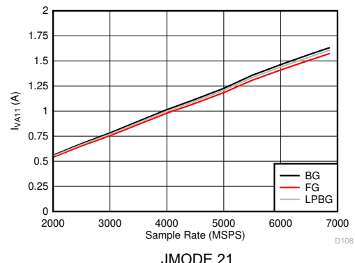
Figure 5-124. DES Mode: I_{VD11} vs Sample Rate
