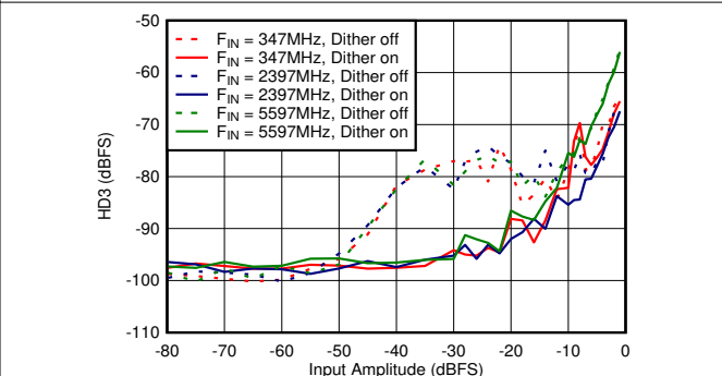
Figure 5-78. Dual Channel Mode: HD3 vs Input Amplitude and Dither
