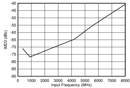
Figure 5-104. Dual Channel Mode: IMD3 vs Input Frequency
