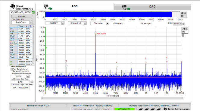
Figure 7-3. FFT for 497.77-MHz Input Signal, 2.7 GSPS, JMODE2
