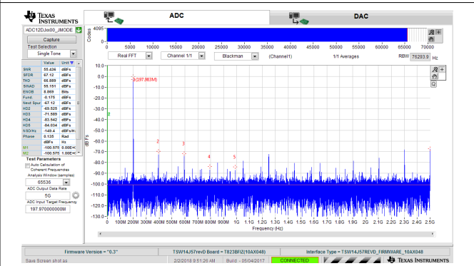
Figure 7-9. 200-MHz, Sine-Wave Frequency Domain (FFT) for 5-GSPS, Single-Channel Oscilloscope
