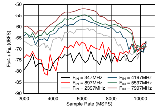
Figure 5-42. DES Mode: F_s/4 + F_{IN} vs Sample Rate and Input Frequency
