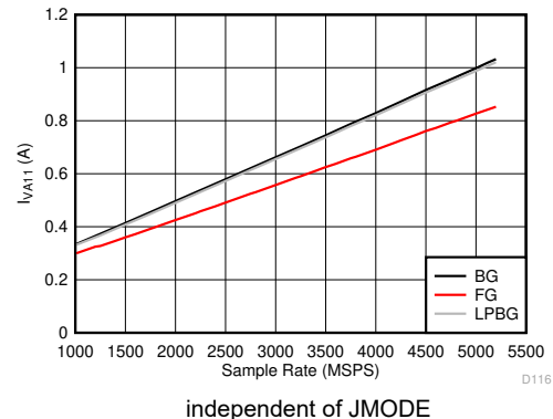
Figure 5-132. Dual Channel Mode: I_{VA11} vs Sample Rate
