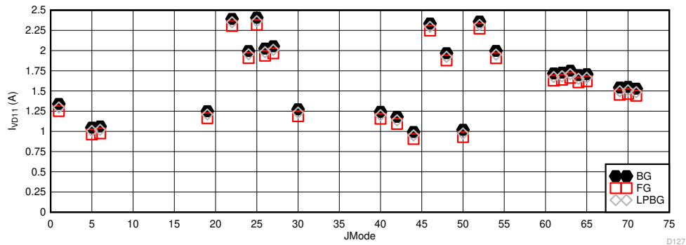
Figure 5-110. DES Mode: I_{VA11} vs \text{JMODE} at 10.4GSPS
