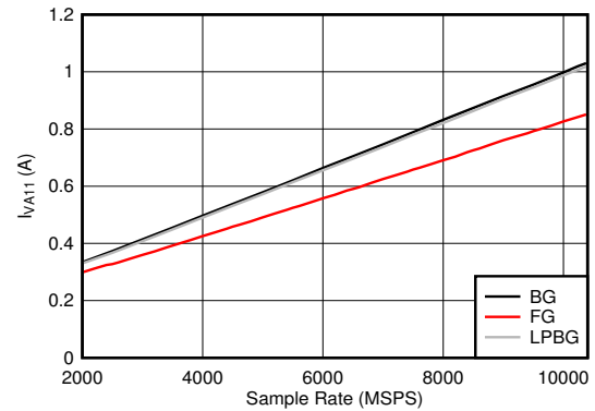
Figure 5-122. DES Mode: I_{VA11} vs Sample Rate
