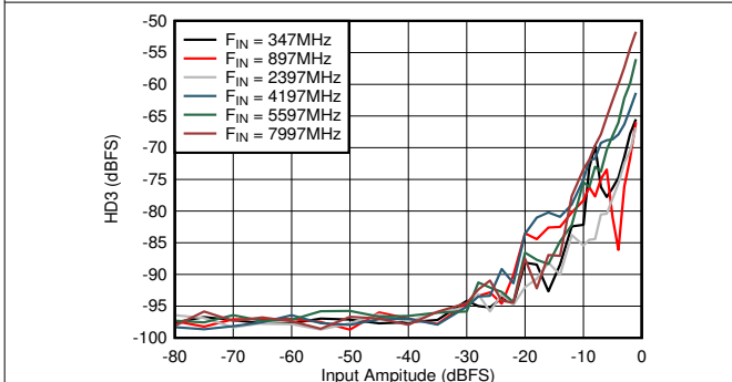
Figure 5-77. Dual Channel Mode: HD3 vs Input Amplitude and Frequency
