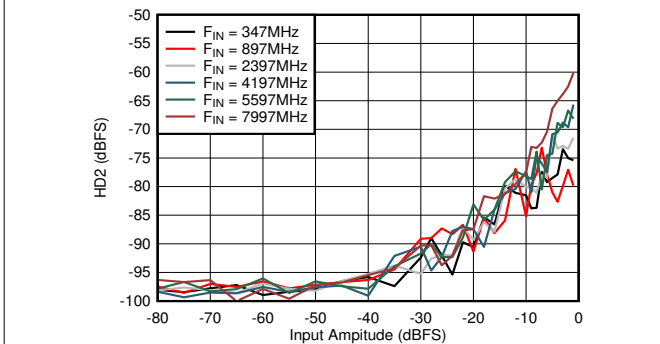
Figure 5-75. Dual Channel Mode: HD2 vs Input Amplitude and Frequency
