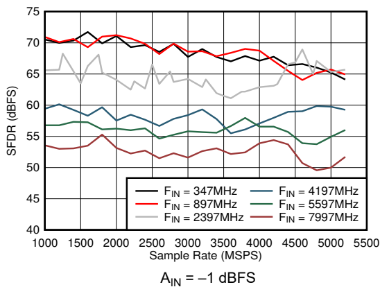
Figure 5-47. Dual Channel Mode: SFDR vs Sample Rate and Input Frequency
