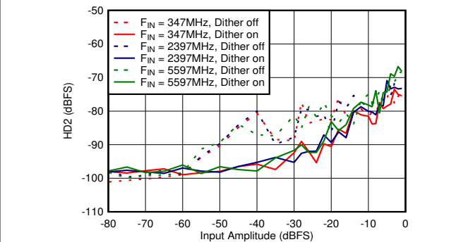
Figure 5-76. Dual Channel Mode: HD2 vs Input Amplitude and Dither
