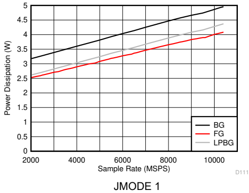
Figure 5-127. DES Mode: Power Dissipation vs Sample Rate
