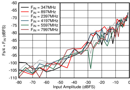
Figure 5-67. DES Mode: F_s/4 + F_{IN} vs Input Amplitude and Frequency
