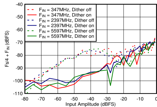
Figure 5-66. DES Mode: F_s/4 + F_{\text{IN}} vs Input Amplitude and Dither
