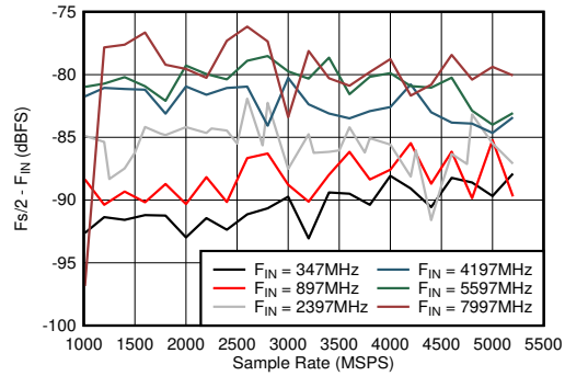
Figure 5-56. Dual Channel Mode: F_s/2 - F_{IN} vs Sample Rate and Input Frequency
