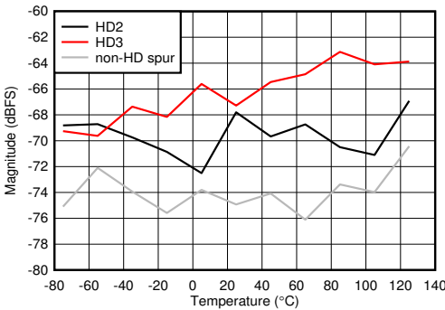
FG calibration at each temperature Figure 5-87. DES Mode: HD2, HD3 and Worst non-HD Spur vs Temperature
