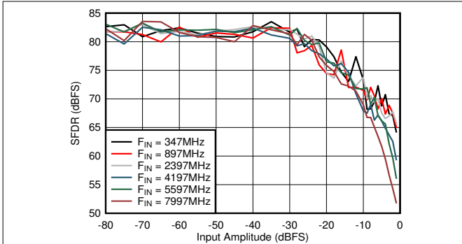
Figure 5-73. Dual Channel Mode: SFDR vs Input Amplitude and Frequency
