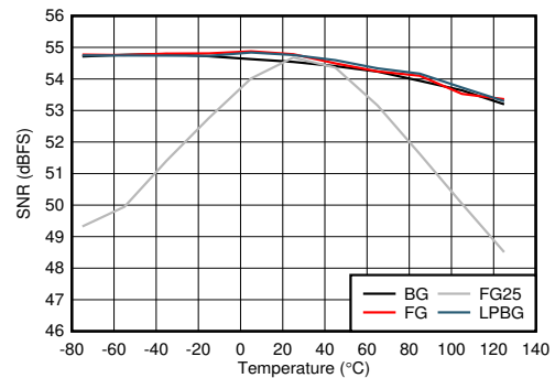
FG25 is calibrated at 25^\circ\text{C} and held at other temperatures, other modes recalibrated at each temperature Figure 5-90. Dual Channel Mode: SNR vs Temperature and Calibration Mode
