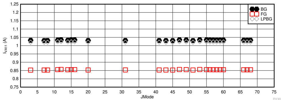
Figure 5-113. Dual Channel Mode: I_{VA19} vs JMODE at 5.2GSPS
