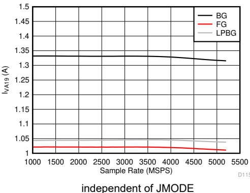
Figure 5-131. Dual Channel Mode: I_{VA19} vs Sample Rate
