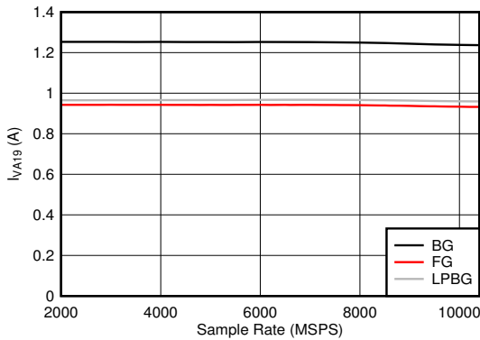
Figure 5-121. DES Mode: I_{VA19} vs Sample Rate
