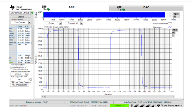
Figure 7-7. 40-MHz, Square-Wave Time Domain for 5-GSPS, Single-Channel Oscilloscope
