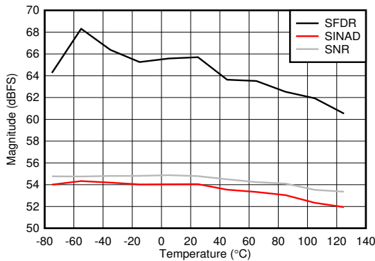
FG calibration at each temperature Figure 5-89. Dual Channel Mode: SNR, SINAD and SFDR vs Temperature
