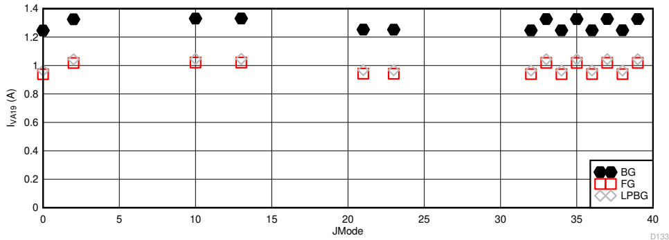
Figure 5-116. Dual Channel Mode: Power Dissipation vs JMODE at 5.2GSPS
