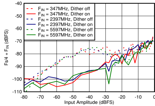
Figure 5-68. DES Mode: F_s/4 + F_{IN} vs Input Amplitude and Dither
