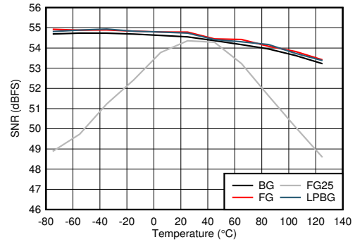
FG25 is calibrated at 25^\circ\text{C} and held at other temperatures, other modes recalibrated at each temperature Figure 5-86. DES Mode: SNR vs Temperature and Calibration Mode
