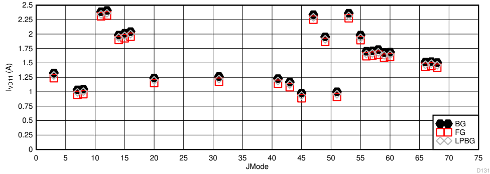
Figure 5-115. Dual Channel Mode: I_{VD11} vs JMODE at 5.2GSPS
