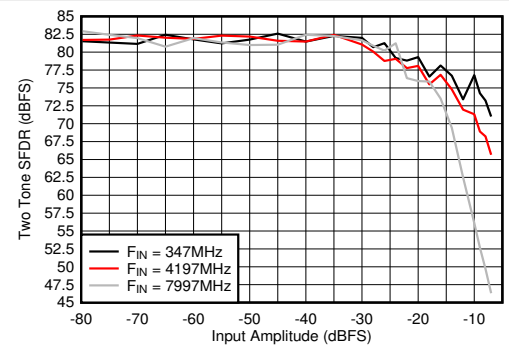
Figure 5-108. Dual Channel Mode: Two Tone SFDR vs Input Amplitude
