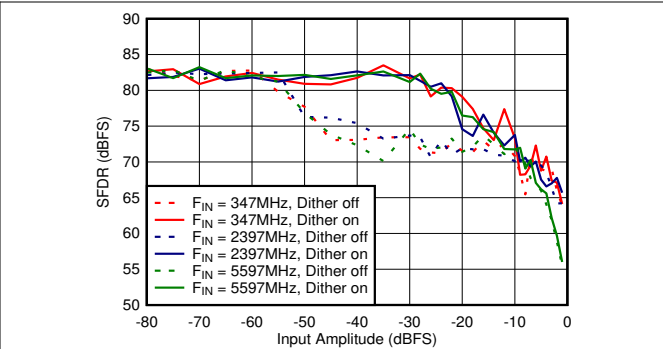
Figure 5-74. Dual Channel Mode: SFDR vs Input Amplitude and Dither
