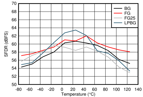
FG25 is calibrated at 25^\circ\text{C} and held at other temperatures, other modes recalibrated at each temperature Figure 5-88. DES Mode: SFDR vs Temperature and Calibration Mode
