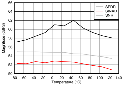
FG calibration at each temperature Figure 5-85. DES Mode: SNR, SINAD and SFDR vs Temperature
