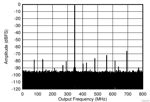
High power mode Figure 5-4. Single Tone FFT at 347 MHz and -1 dBFS
