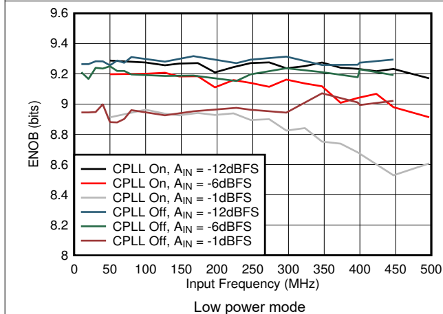
Figure 5-57. ENOB vs A_{IN} and C-PLL
