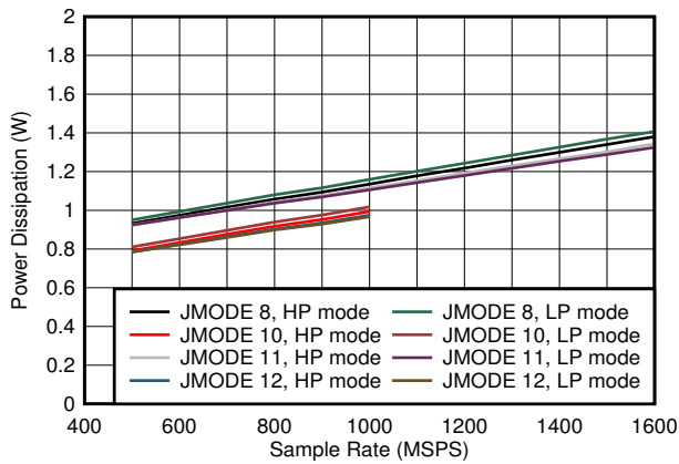
Low power background calibration mode Figure 5-101. Single Channel, Power Dissipation vs F_S and JMODE 8 - 12
