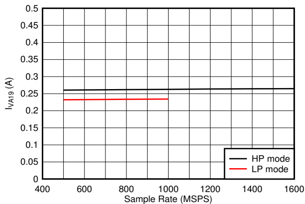
Low power background calibration mode, independent of JMODE Figure 5-103. Single Channel, I_{VA19} vs F_S
