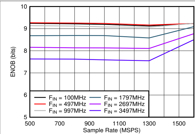
Figure 5-26. ENOB vs Sample Rate
