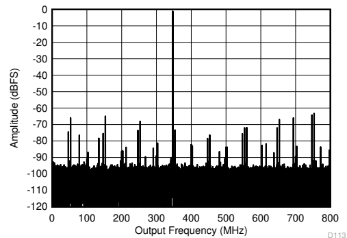
High power mode, C-PLL on, Noise suppression off Figure 5-6. Single Tone FFT at 347 MHz and -1 dBFS
