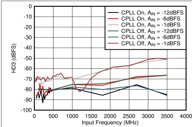
Figure 5-53. HD3 vs A_{IN} and C-PLL
