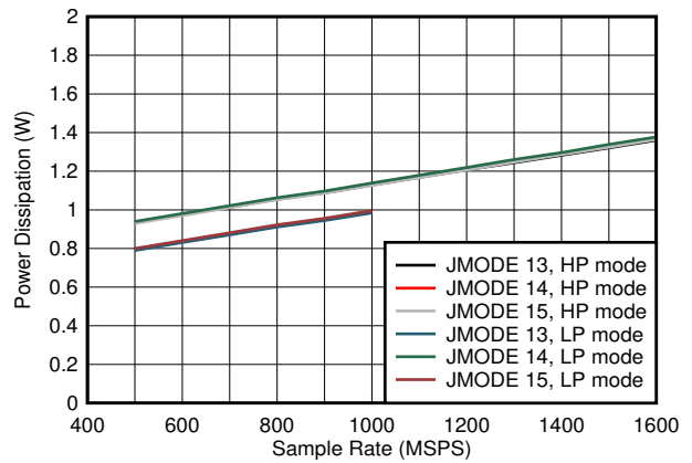
Low power background calibration mode Figure 5-102. Single Channel, Power Dissipation vs F_S and JMODE 13 - 15
