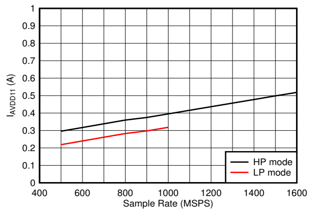
Low power background calibration mode, independent of JMODE Figure 5-104. Single Channel, I_{VA11} vs F_S
