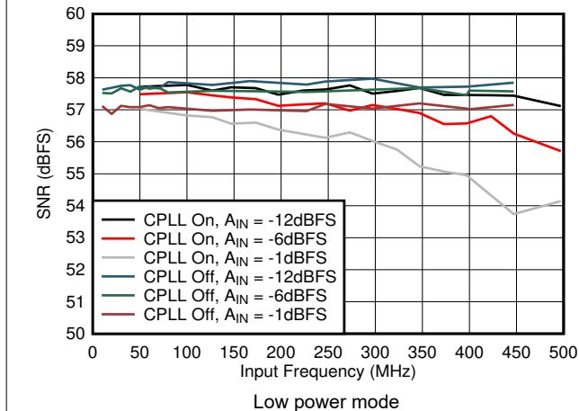
Figure 5-55. SNR vs A_{IN} and C-PLL
