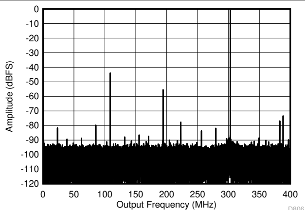
Figure 7-12. Single Tone FFT at 2097 MHz and -1dBFS Low Power Mode
