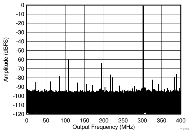
Figure 7-8. Single Tone FFT at 2097 MHz and -1dBFS
