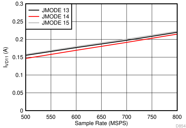
Figure 7-97. Dual Channel, I_{VD11} vs F_S for JMODES 13 - 15
