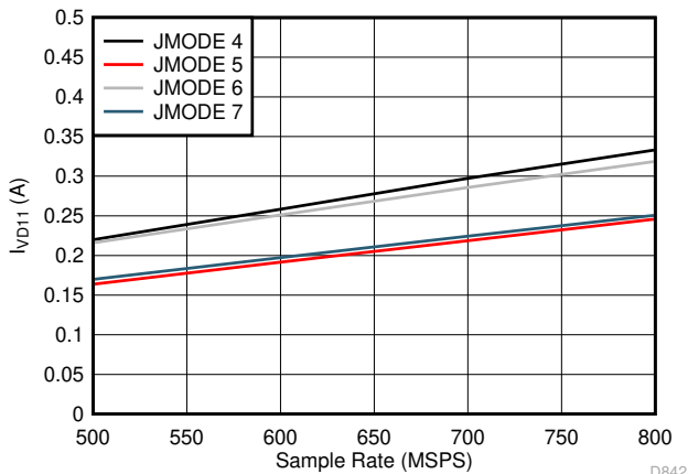
Independent of Power Mode Figure 7-81. Quad Channel, I_{VDD11} vs F_S for JMODES 4 - 7
