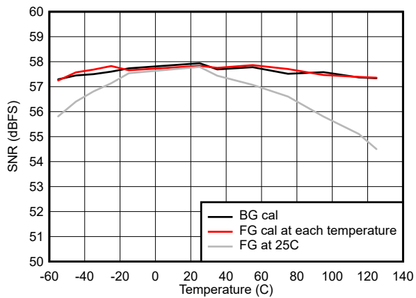
Figure 7-43. SNR vs Temperature
