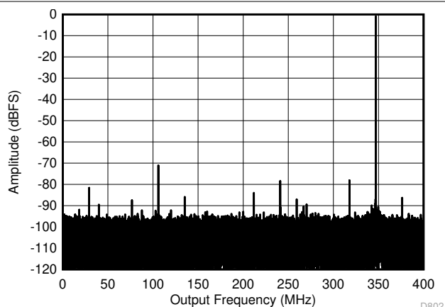
Figure 7-10. Single Tone FFT at 347 MHz and -1dBFS Low Power Mode
