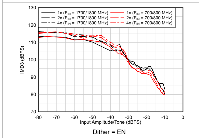
Figure 6-35. IMD3 Performance vs A_{IN}
