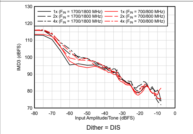
Figure 6-34. IMD3 Performance vs A_{IN}
