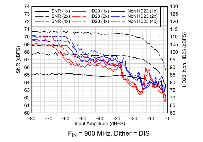
Figure 6-32. AC Performance vs A_{IN}
