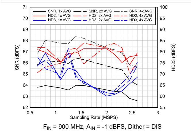
Figure 6-36. AC Performance vs F_S
