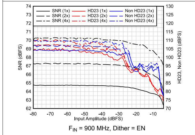
Figure 6-33. AC Performance vs A_{IN}
