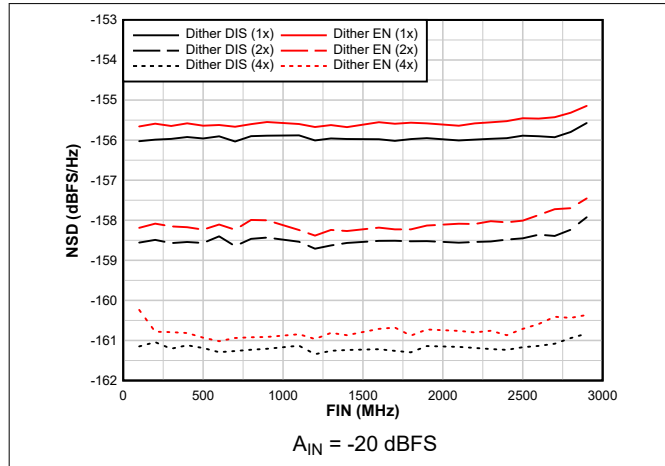
Figure 6-31. NSD Performance vs F_{IN}
