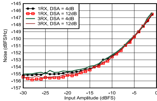
Figure 6-320. RX Noise Spectral Density vs Input Amplitude and Channel at 1.75 GHz
