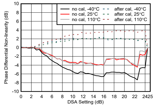
Figure 6-417. RX Phase Differential Nonlinearity at 8.1 GHz
