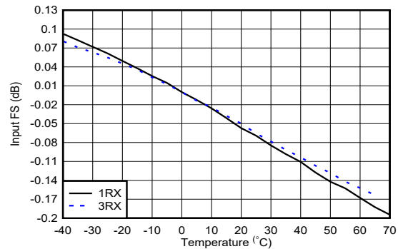
Figure 6-276. RX Input Fullscale vs Temperature and Channel at 800 MHz
