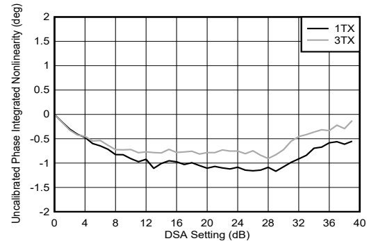
Figure 6-197. TX DSA Uncalibrated Phase Integrated Nonlinearity at 8.11 GHz
