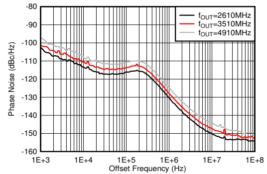
Figure 6-483. Phase Noise for 10-GHz VCO vs Offset Frequency and f_{OUT} at 25°C
