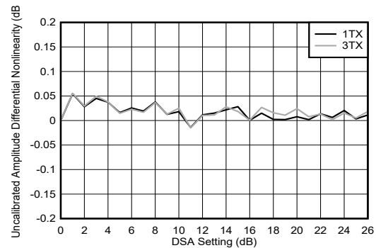
Figure 6-230. TX DSA Uncalibrated Amplitude Differential Nonlinearity
