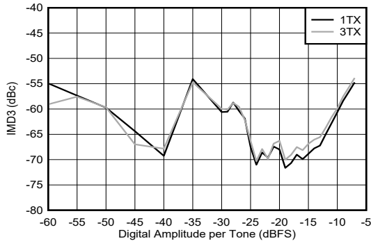
-7 dBFS each tone, 50 MHz tone spacing
