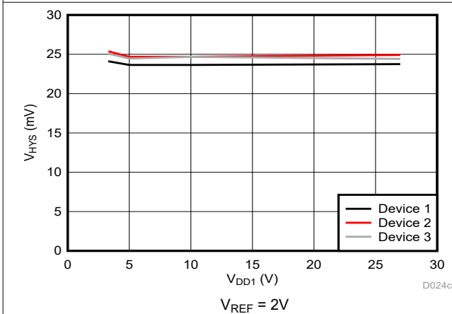
Figure 5-22. Trip Threshold Hysteresis vs Supply Voltage
