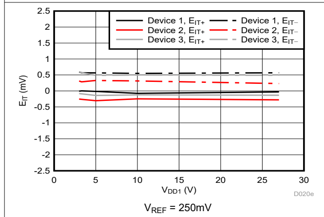
Figure 5-14. Trip Threshold Error vs Supply Voltage
