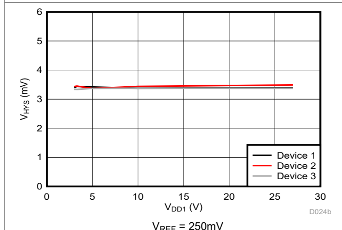
Figure 5-16. Trip Threshold Hysteresis vs Supply Voltage
