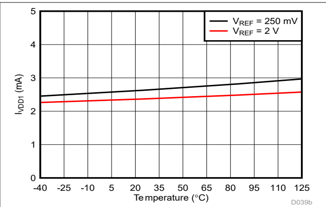
Figure 5-31. High-Side Supply Current vs Temperature
