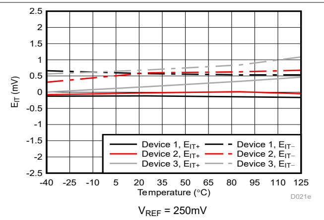
Figure 5-15. Trip Threshold Error vs Temperature
