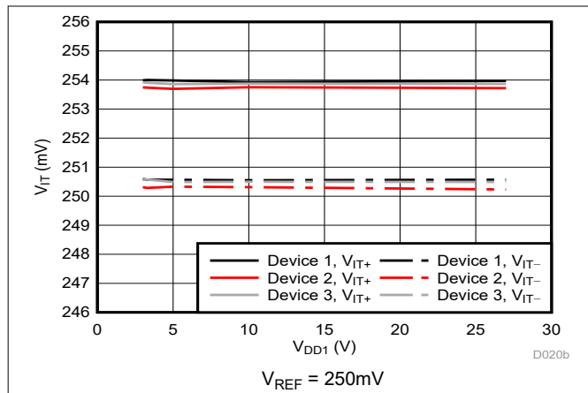
Figure 5-12. Trip Threshold vs Supply Voltage
