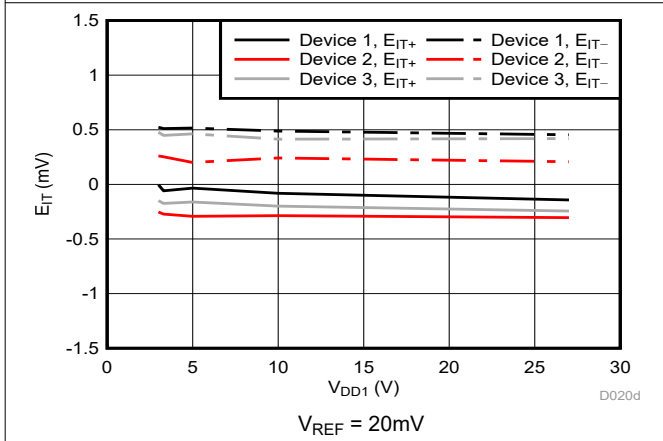
Figure 5-8. Trip Threshold Error vs Supply Voltage
