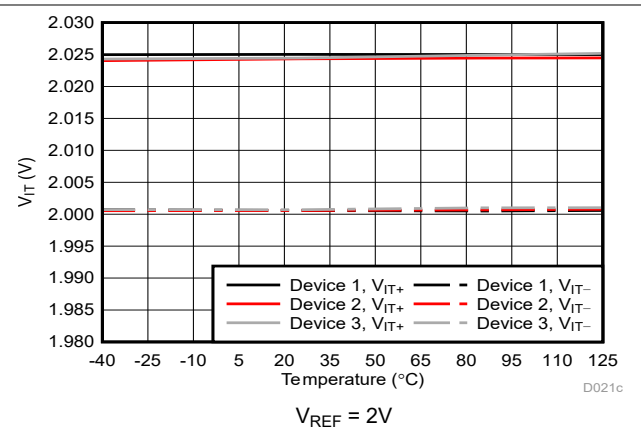
Figure 5-19. Trip Threshold vs Temperature
