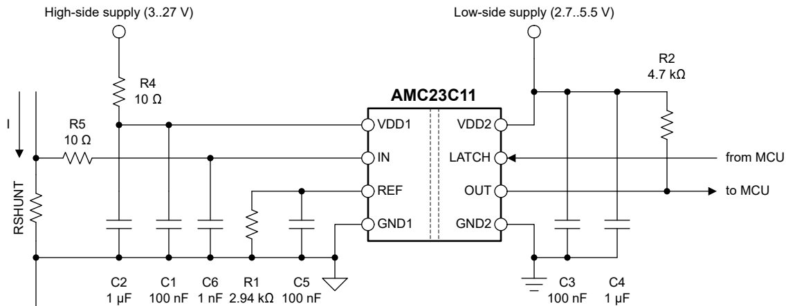
Figure 7-4. Decoupling of the AMC23C11
