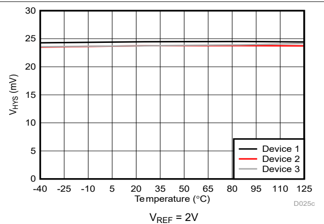
Figure 5-23. Trip Threshold Hysteresis vs Temperature
