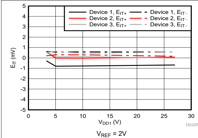
Figure 5-20. Trip Threshold Error vs Supply Voltage
