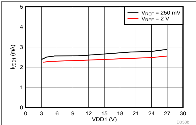
Figure 5-30. High-Side Supply Current vs Supply Voltage
