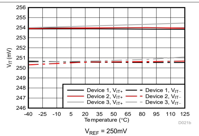
Figure 5-13. Trip Threshold vs Temperature
