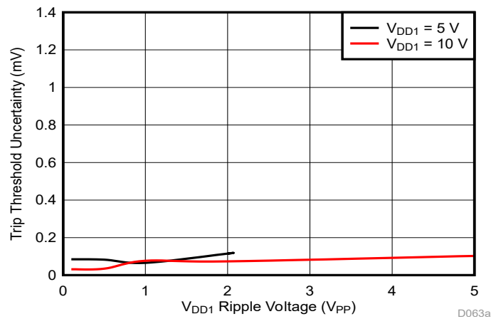
Figure 7-3. Trip Threshold Sensitivity to VDD1 Ripple Voltage (f RIPLLE = 10kHz)
