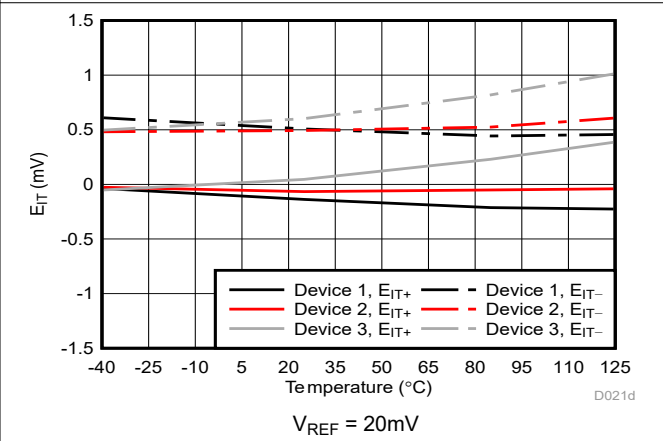
Figure 5-9. Trip Threshold Error vs Temperature
