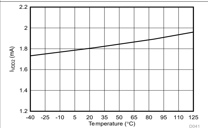
Figure 5-31. High-Side Supply Current vs Temperature
