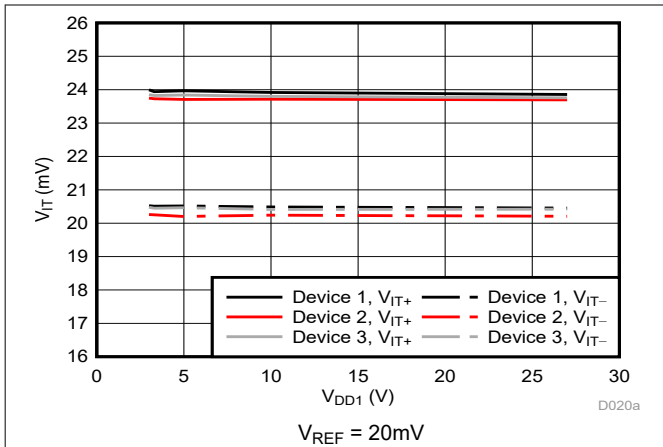
Figure 5-6. Trip Threshold vs Supply Voltage
