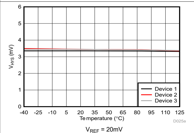
Figure 5-11. Trip Threshold Hysteresis vs Temperature
