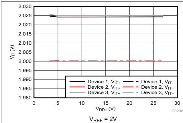
Figure 5-18. Trip Threshold vs Supply Voltage
