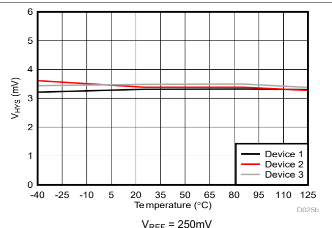
Figure 5-17. Trip Threshold Hysteresis vs Temperature
