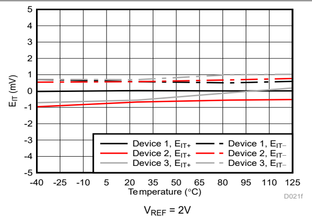
Figure 5-21. Trip Threshold Error vs Temperature
