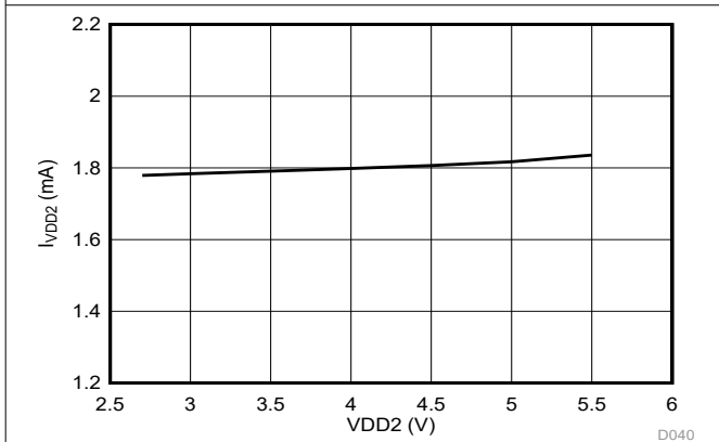
Figure 5-30. High-Side Supply Current vs Supply Voltage
