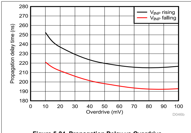
Figure 5-24. Propagation Delay vs Overdrive
