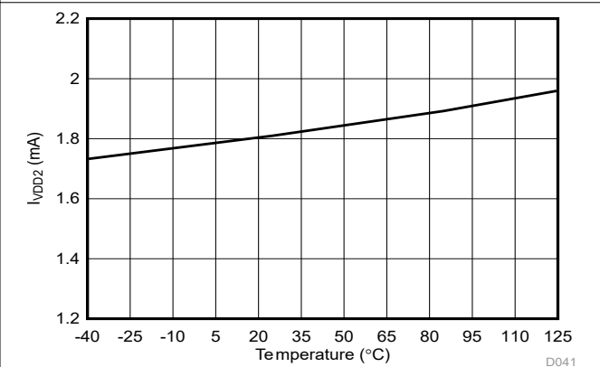
Figure 5-61. High-Side Supply Current vs Temperature
