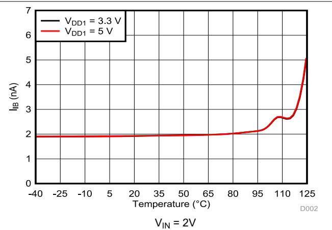
Figure 5-57. Input Bias Current vs Temperature
