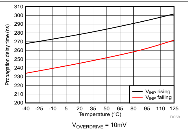
Figure 5-55. Cmp1 Propagation Delay vs Temperature
