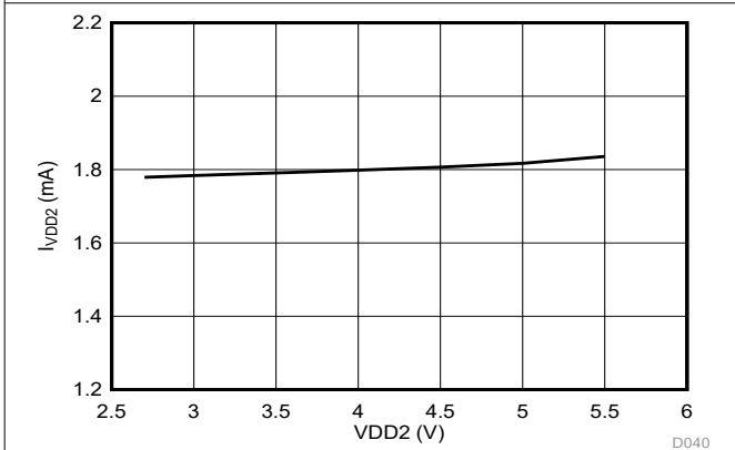
Figure 5-60. High-Side Supply Current vs Supply Voltage
