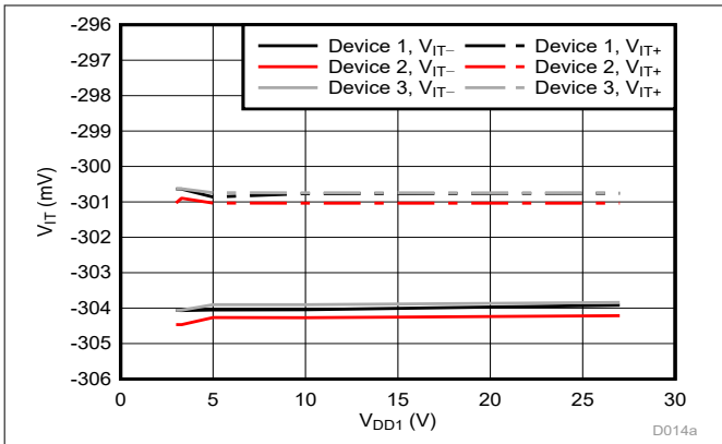
Figure 5-12. Cmp3 Trip Threshold vs Supply Voltage
