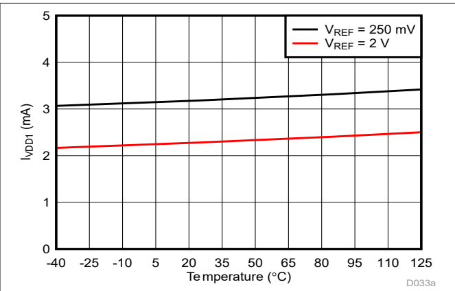
Figure 5-61. High-Side Supply Current vs Temperature
