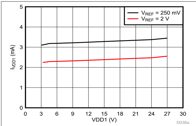
Figure 5-60. High-Side Supply Current vs Supply Voltage
