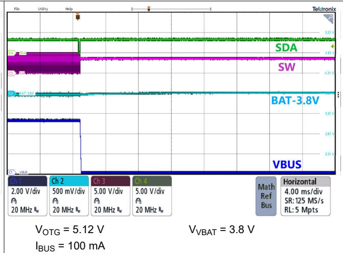
Figure 8-9. Boost Mode Power Down
