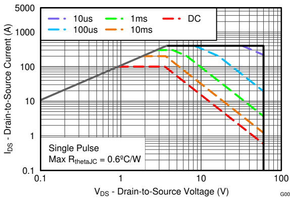
Figure 3-10. Maximum Safe Operating Area
