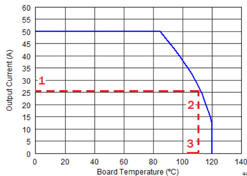
Figure 34. Power Block SOA
