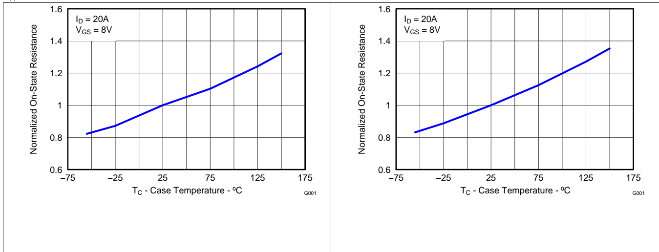
Figure 23. Control MOSFET Normalized R_{DS(on)}
