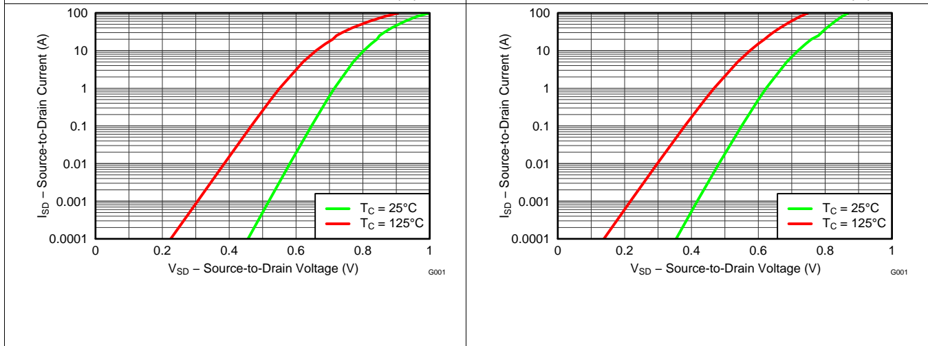
Figure 25. Control MOSFET Body Diode
