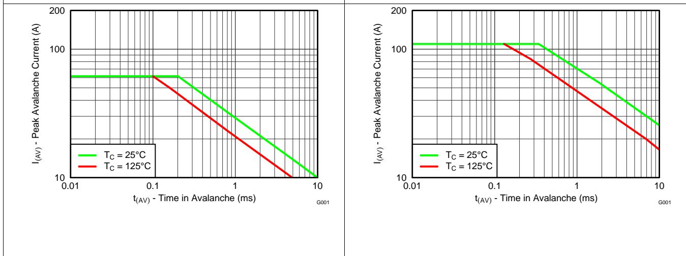
Figure 27. Control MOSFET Unclamped Inductive Switching
