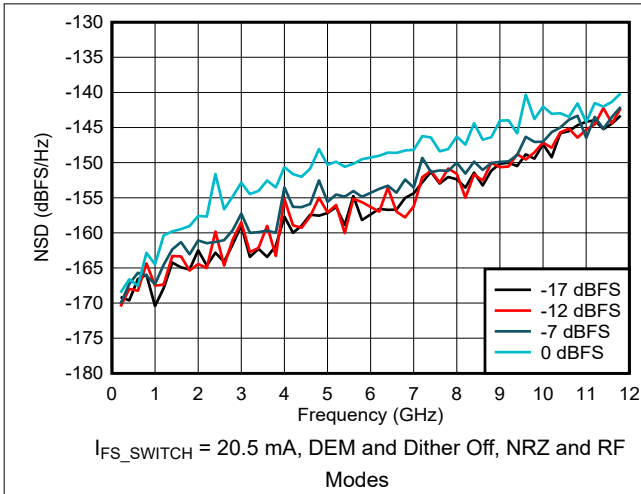
Figure 6-64. NSD vs Output Frequency and Digital Amplitude
