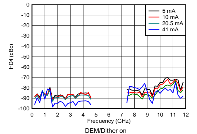
Figure 6-169. HD4 vs Frequency and Output Current in DES2X Modes
