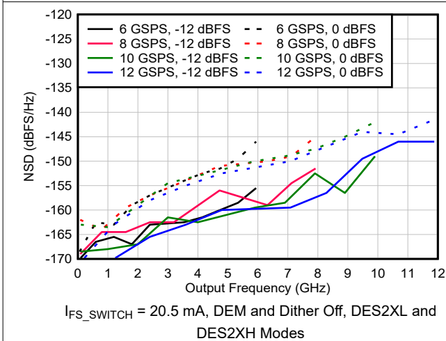
Figure 6-74. NSD vs Output Frequency and Sample Rate
