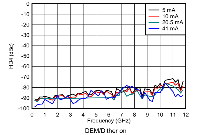
Figure 6-167. HD4 vs Frequency and Output Current in NRZ/RF Modes
