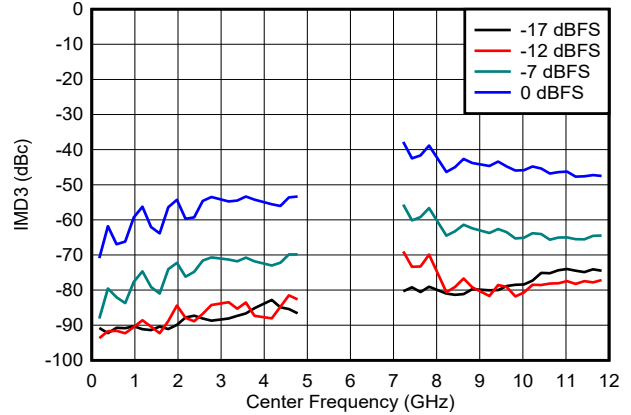
Figure 6-117. IMD3 vs Frequency and Digital Amplitude in DES2X Modes
