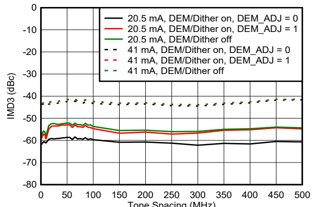
Figure 6-119. IMD3 vs Tone Spacing in DES2XL Mode
