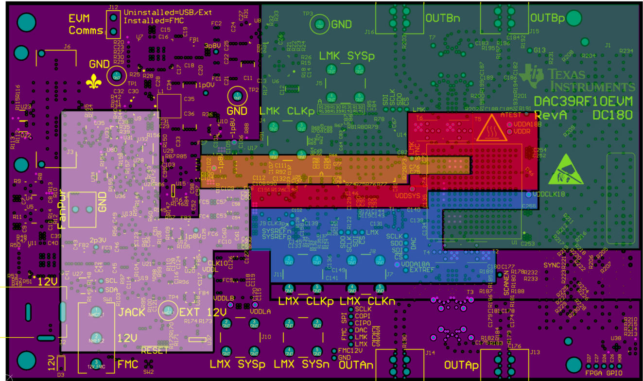
Layer12 / PWR3 DAC VDDA18A = RED DAC VDDA18B = ORANGE DAC VDDDB = YELLOW DAC VEExA = GREEN DAC VEExB = BLUE VDDIO = WHITE
