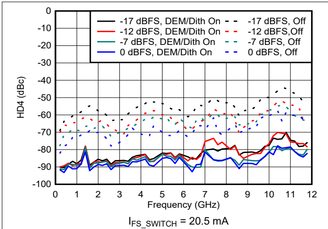
Figure 6-170. HD4 vs Frequency and Digital Amplitude in NRZ/RF Modes
