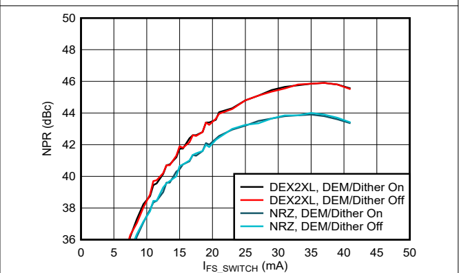
Figure 6-192. Noise Power Ratio vs Output Current: 2 nd Nyquist Zone
