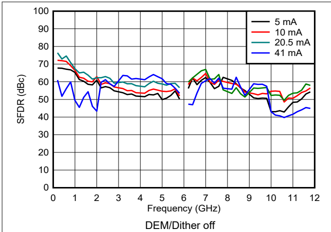
Figure 6-92. SFDR vs Frequency and Output Current in DES2X Modes
