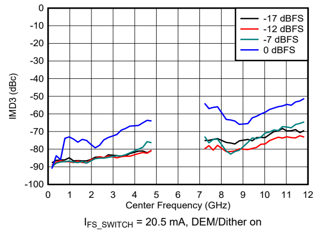
Figure 6-115. IMD3 vs Frequency and Digital Amplitude in DES2X Modes
