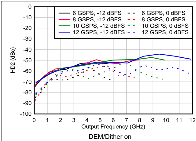
Figure 6-146. HD2 vs Frequency and Sample Rate in NRZ/RF Modes
