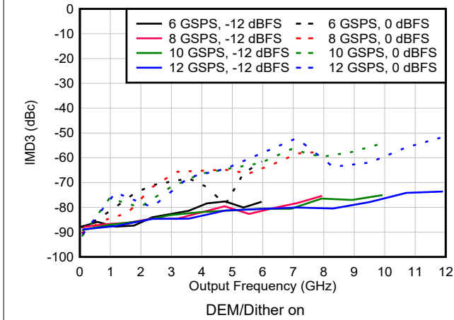
Figure 6-124. IMD3 vs Frequency and Sample Rate in DES2X Modes
