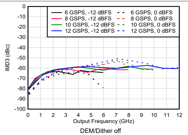
Figure 6-123. IMD3 vs Frequency and Sample Rate in NRZ/RF Modes
