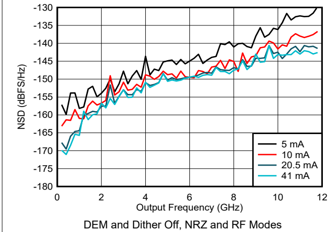
Figure 6-60. NSD vs Output Frequency and Output Current
