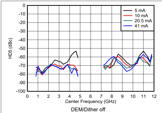
Figure 6-176. HD5 vs Frequency and Output Current in DES2X Modes
