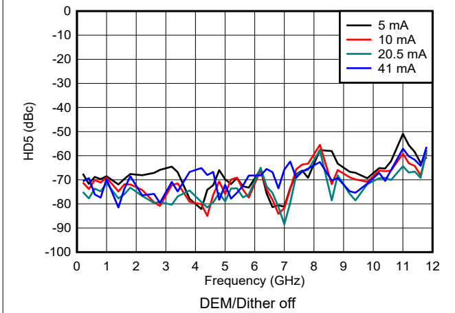
Figure 6-174. HD5 vs Frequency and Output Current in NRZ/RF Modes
