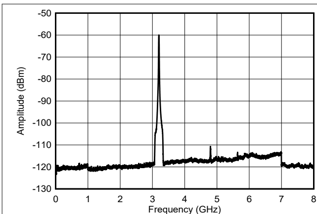
Figure 8-17. NLFM Chirp Output Spectra across 0 - 8 GHz
