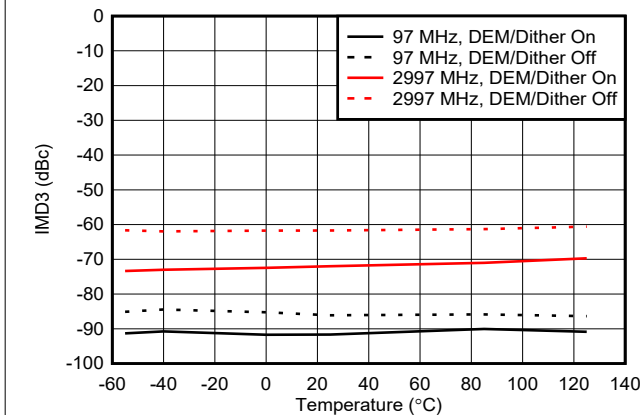
Figure 6-126. IMD3 vs Temperature in NRZ Mode
