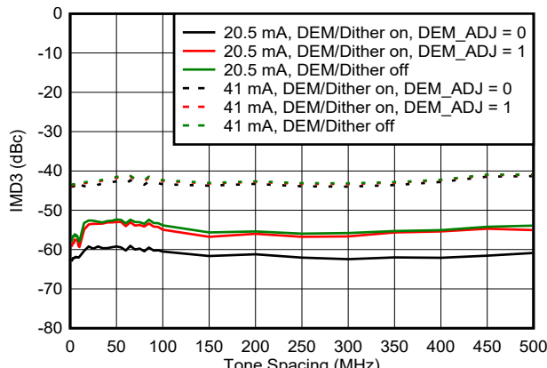
Figure 6-118. IMD3 vs Tone Spacing in NRZ Mode
