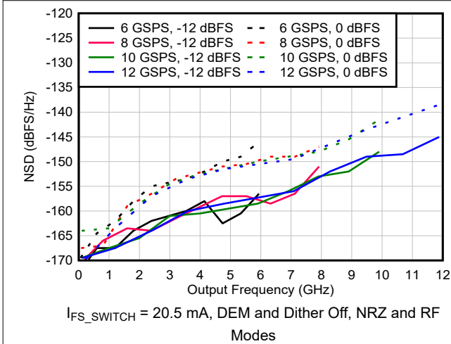
Figure 6-72. NSD vs Output Frequency and Sample Rate
