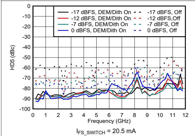
Figure 6-178. HD5 vs Frequency and Digital Amplitude in NRZ/RF Modes
