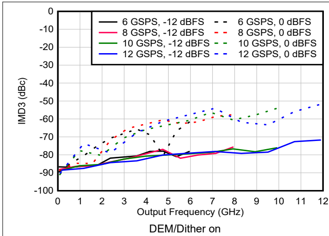
Figure 6-122. IMD3 vs Frequency and Sample Rate in NRZ/RF Modes
