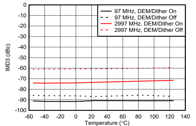
Figure 6-127. IMD3 vs Temperature in DES2XL Mode
