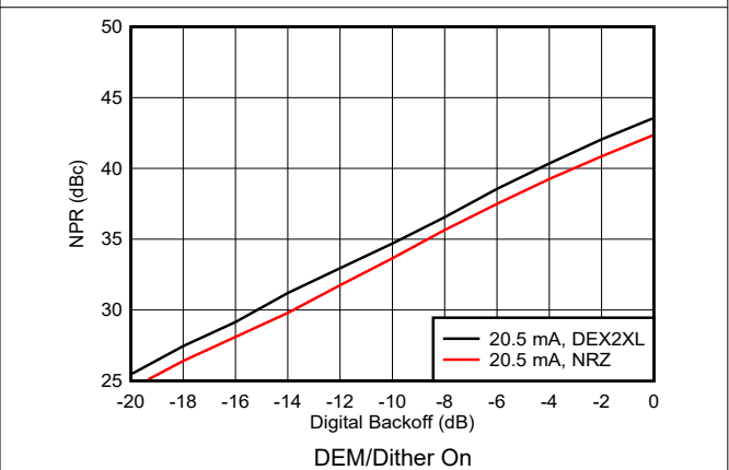
Figure 6-190. Noise Power Ratio vs Digital Backoff: 2 nd Nyquist Zone
