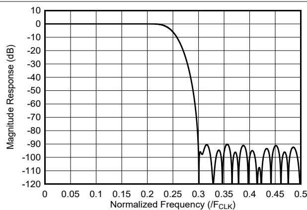
Figure 7-14. 2x Interpolation Filter Response
