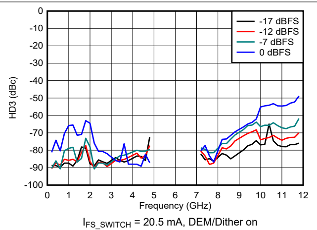
Figure 6-159. HD3 vs Frequency and Digital Amplitude in DES2X Modes
