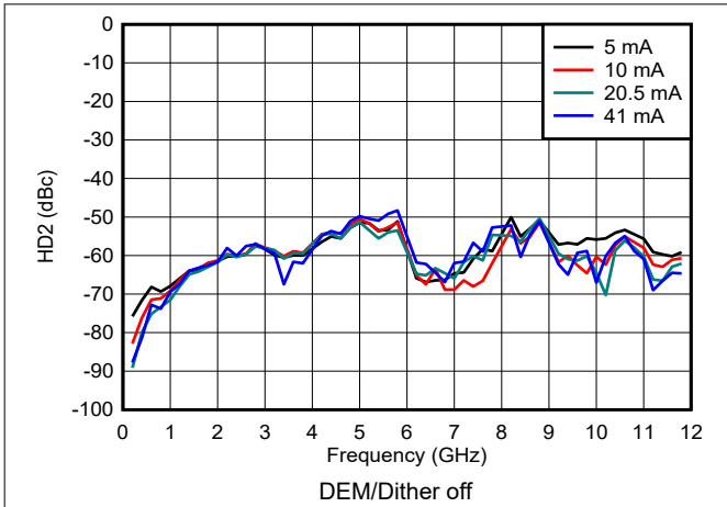
Figure 6-134. HD2 vs Frequency and Output Current in NRZ/RF Modes
