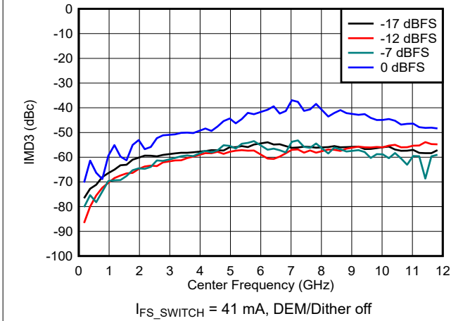
Figure 6-112. IMD3 vs Frequency and Digital Amplitude in NRZ/RF Modes
