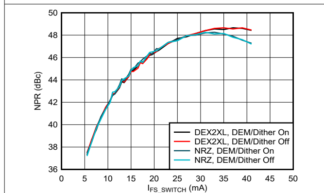
Figure 6-191. Noise Power Ratio vs Output Current: 1 st Nyquist Zone
