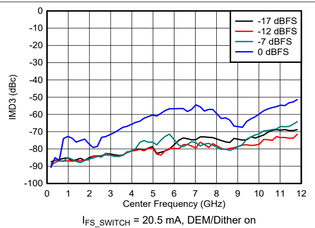
Figure 6-111. IMD3 vs Frequency and Digital Amplitude in NRZ/RF Modes
