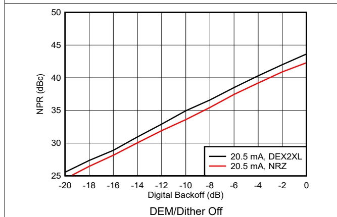
Figure 6-189. Noise Power Ratio vs Digital Backoff: 2 nd Nyquist Zone
