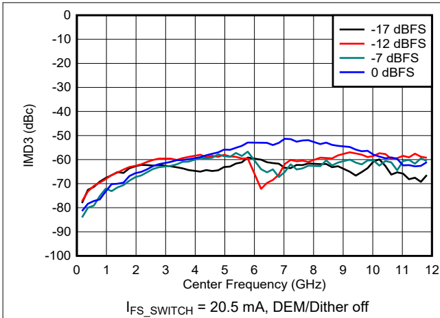
Figure 6-110. IMD3 vs Frequency and Digital Amplitude in NRZ/RF Modes
