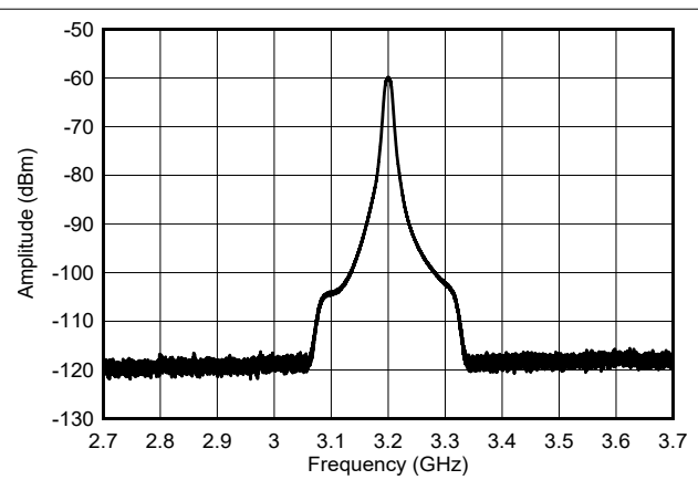
Figure 8-18. NLFM Chirp Output Spectra across 1 GHz
