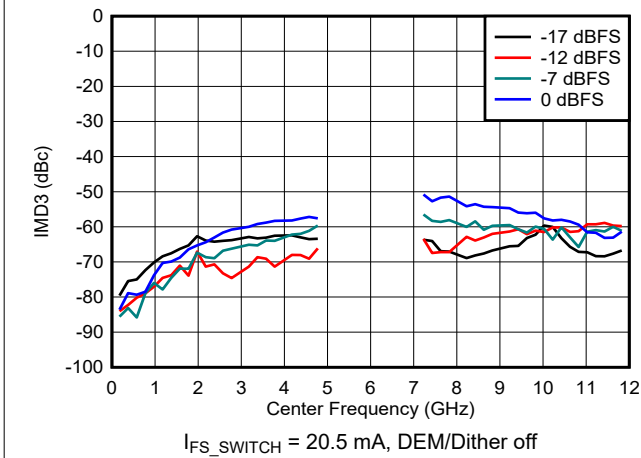
Figure 6-114. IMD3 vs Frequency and Digital Amplitude in DES2X Modes
