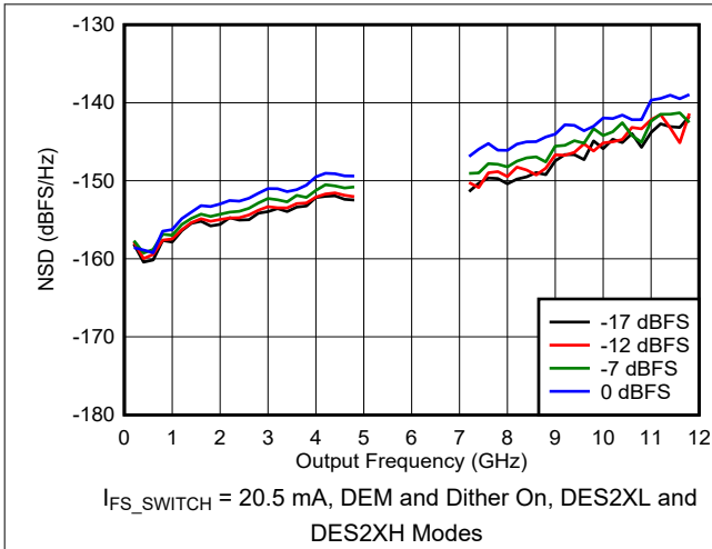
Figure 6-70. NSD vs Output Frequency and Digital Amplitude
