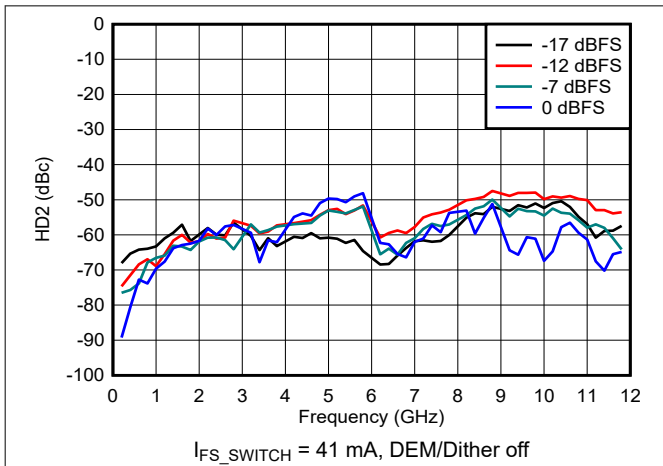
Figure 6-140. HD2 vs Frequency and Digital Amplitude in NRZ/RF Modes
