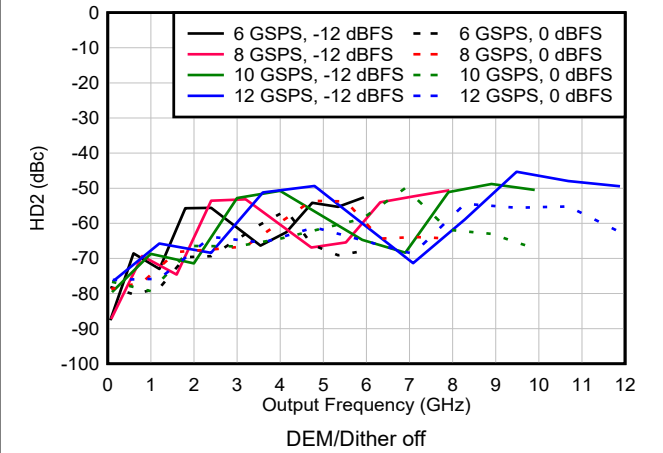
Figure 6-149. HD2 vs Frequency and Sample Rate in DES2X Modes
