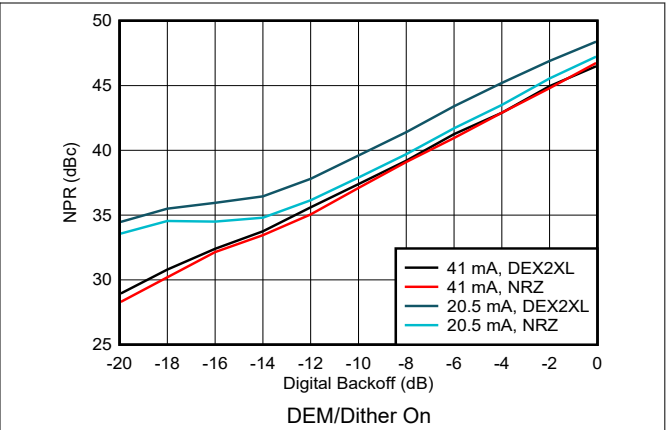
Figure 6-188. Noise Power Ratio vs Digital Backoff: 1 st Nyquist Zone
