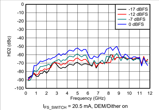
Figure 6-139. HD2 vs Frequency and Digital Amplitude in NRZ/RF Modes
