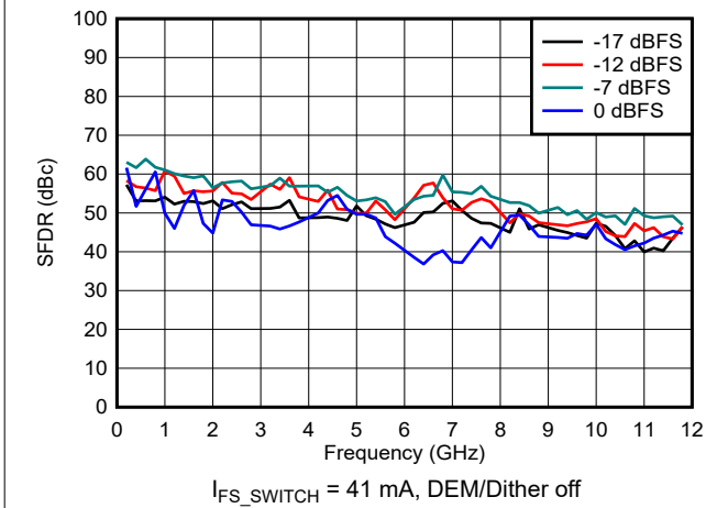
Figure 6-96. SFDR vs Frequency and Digital Amplitude in NRZ/RF Modes
