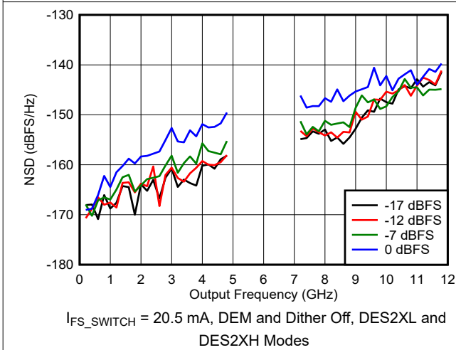
Figure 6-68. NSD vs Output Frequency and Digital Amplitude
