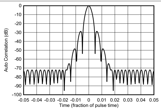
Figure 8-16. Auto-correlation of NLFM Chirp
