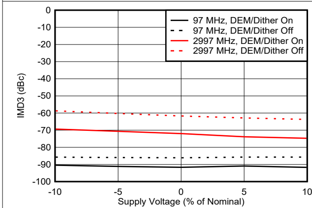
Figure 6-130. IMD3 vs Voltage in NRZ Mode
