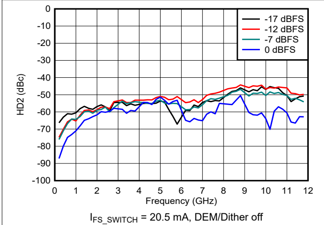
Figure 6-138. HD2 vs Frequency and Digital Amplitude in NRZ/RF Modes
