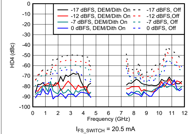
Figure 6-172. HD4 vs Frequency and Digital Amplitude in NRZ/RF Modes
