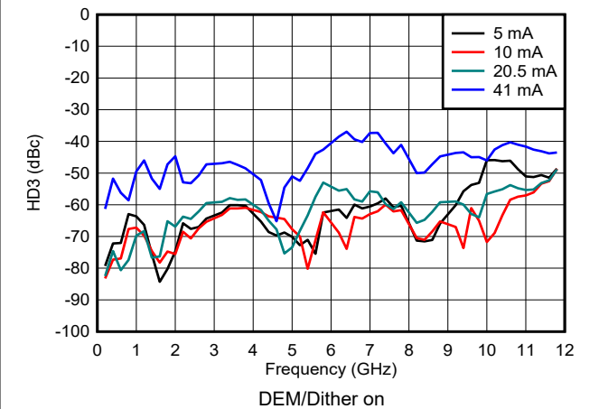
Figure 6-151. HD3 vs Frequency and Output Current in NRZ/RF Modes
