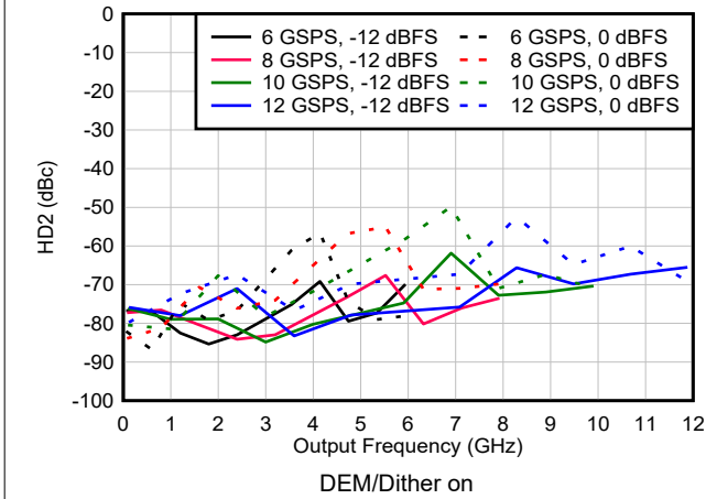
Figure 6-148. HD2 vs Frequency and Sample Rate in DES2X Modes
