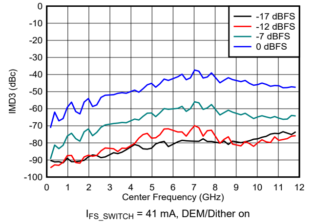
Figure 6-113. IMD3 vs Frequency and Digital Amplitude in NRZ/RF Modes
