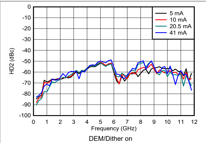
Figure 6-135. HD2 vs Frequency and Output Current in NRZ/RF Modes
