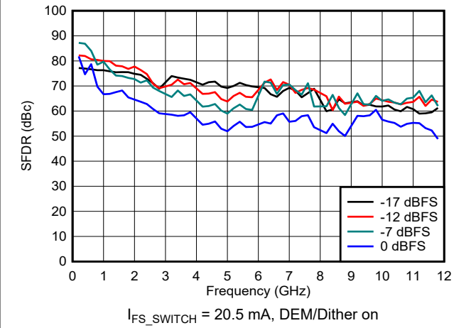
Figure 6-95. SFDR vs Frequency and Digital Amplitude in NRZ/RF Modes
