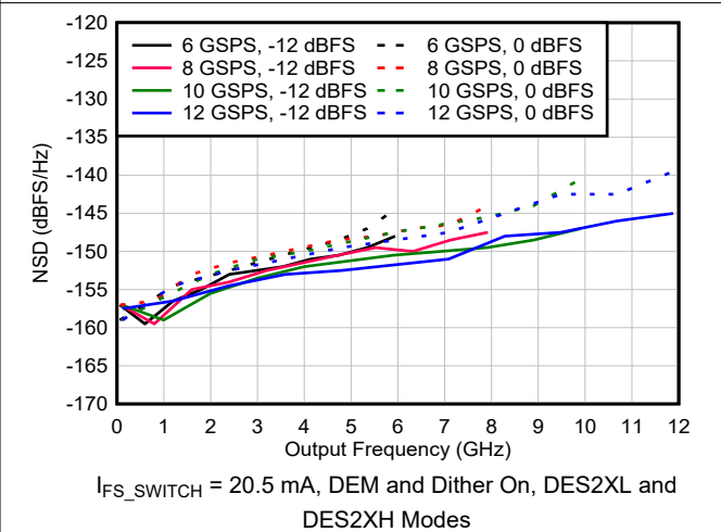
Figure 6-75. NSD vs Output Frequency and Sample Rate
