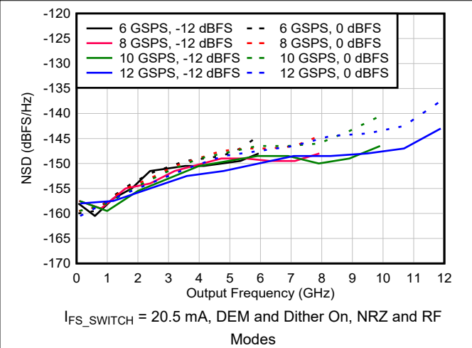
Figure 6-73. NSD vs Output Frequency and Sample Rate
