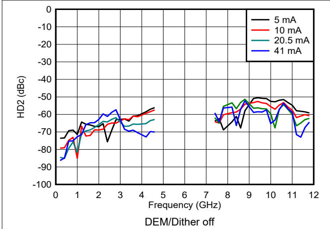
Figure 6-136. HD2 vs Frequency and Output Current in DES2X Modes
