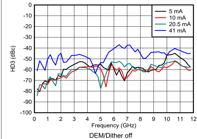
Figure 6-150. HD3 vs Frequency and Output Current in NRZ/RF Modes
