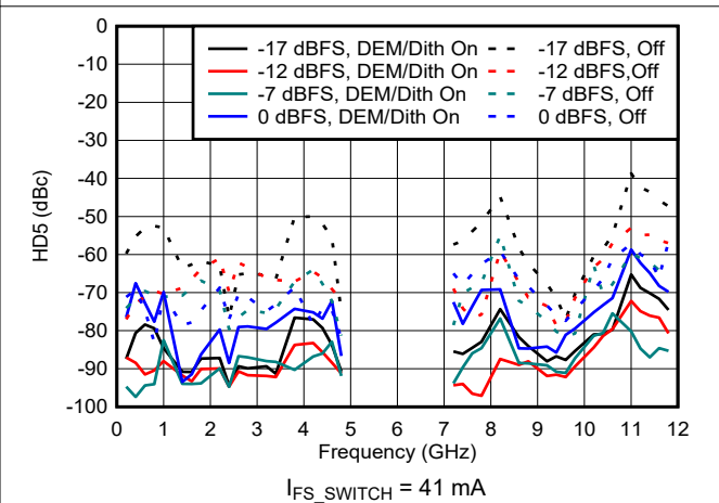
Figure 6-181. HD5 vs Frequency and Digital Amplitude in DES2X Modes
