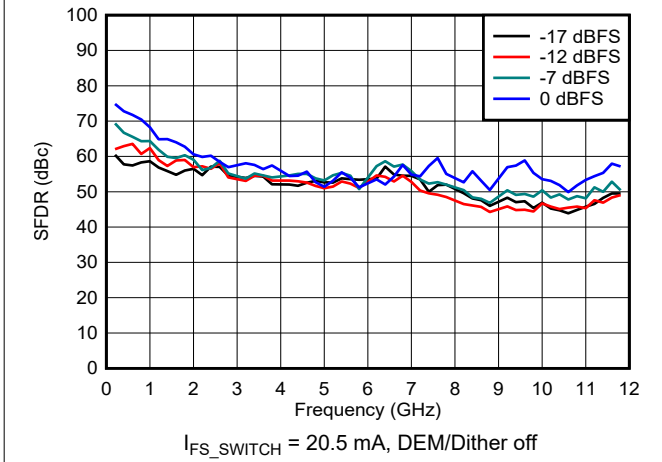
Figure 6-94. SFDR vs Frequency and Digital Amplitude in NRZ/RF Modes
