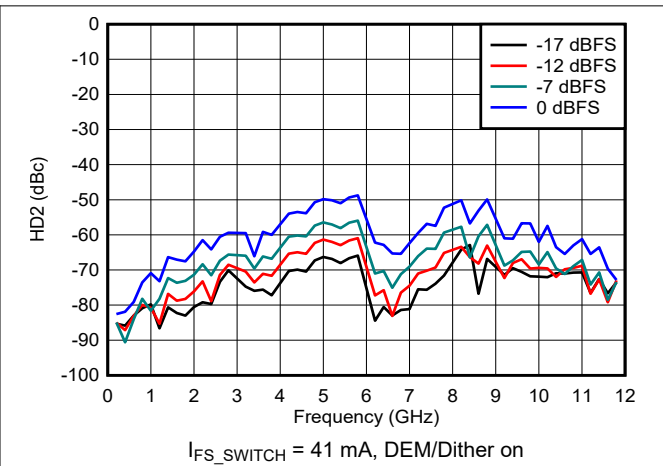
Figure 6-141. HD2 vs Frequency and Digital Amplitude in NRZ/RF Modes
