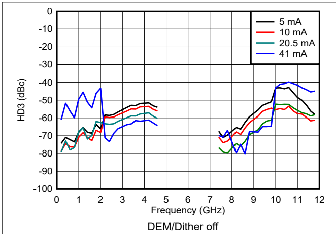
Figure 6-152. HD3 vs Frequency and Output Current in DES2X Modes
