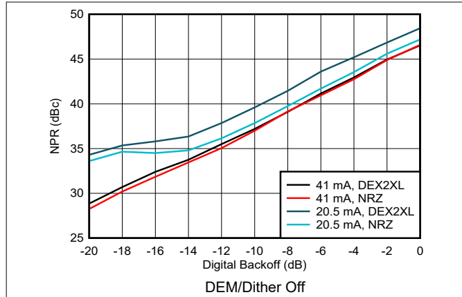
Figure 6-187. Noise Power Ratio vs Digital Backoff: 1 st Nyquist Zone
