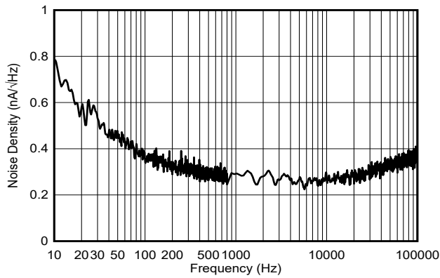
Figure 6-55. Current Output Noise Density
