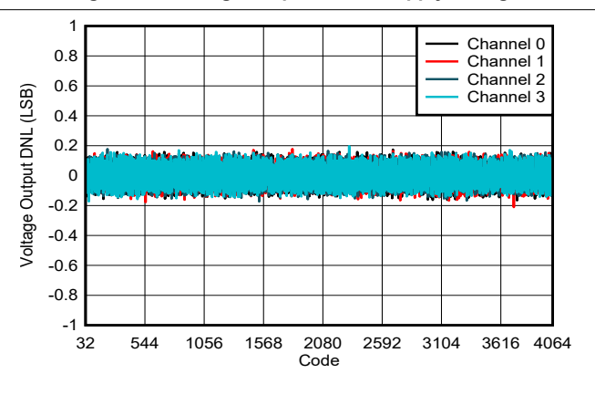
Figure 6-9. Voltage Output DNL vs Digital Input Code
