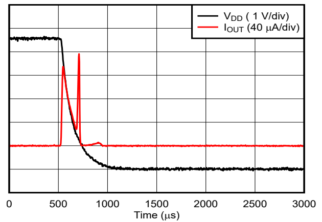
DAC at mid scale ( 0\ \mu\text{A} ) Figure 6-52. Current Output Power-Off Glitch
