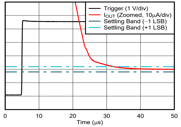
Figure 6-50. Current Output Settling Time: Falling Edge ( \frac{1}{4} to \frac{3}{4} scale)
