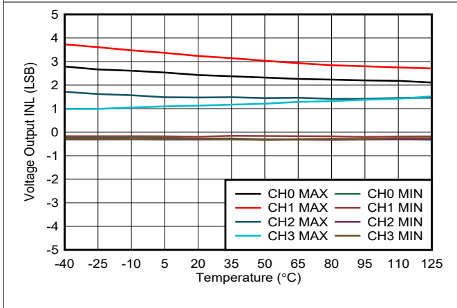
Figure 6-6. Voltage Output INL vs Temperature
