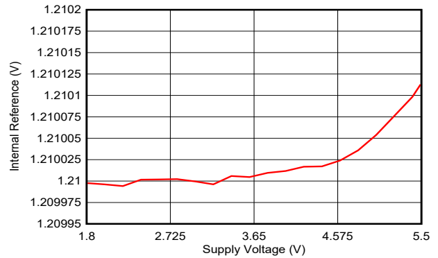
Figure 6-63. Internal Reference vs Supply Voltage
