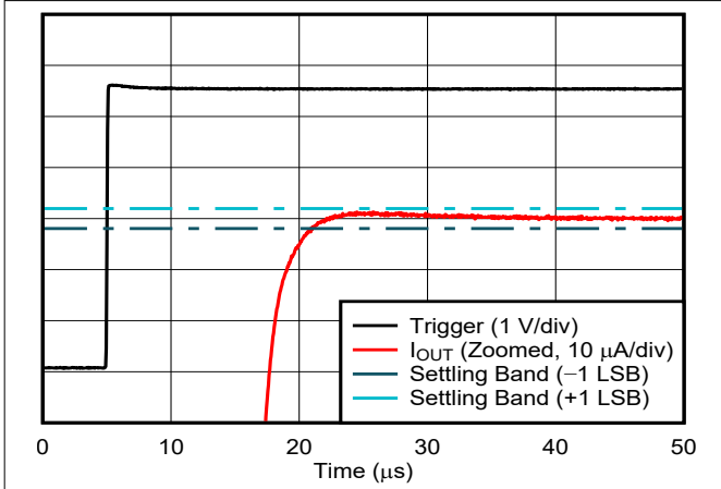
Figure 6-49. Current Output Settling Time: Rising Edge ( \frac{1}{4} to \frac{3}{4} scale)
