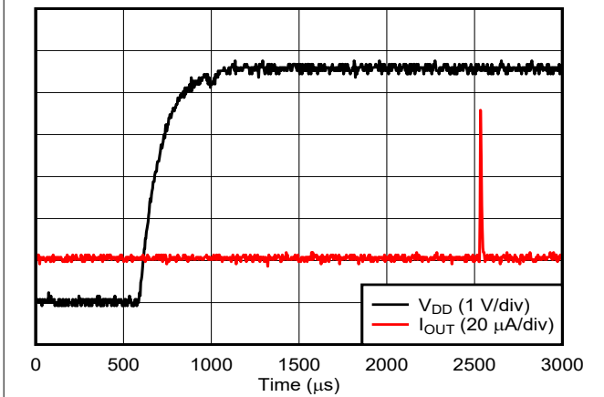
DAC at mid scale ( 0\ \mu\text{A} ) stored in EEPROM Figure 6-51. Current Output Power-On Glitch
