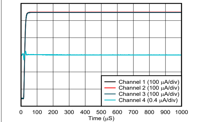
Channel 4 is resident, all other channels are interferers Figure 6-53. Current Output Channel-to-Channel Crosstalk
