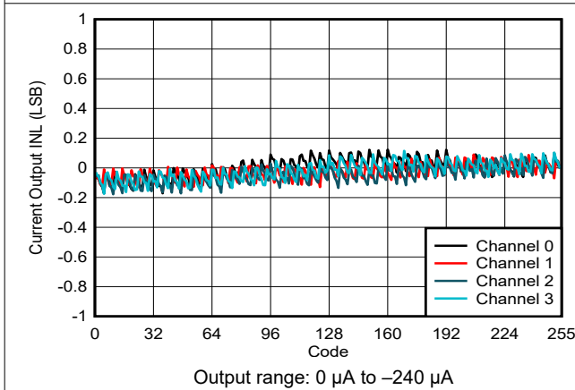
Figure 6-33. Current Output INL vs Digital Input Code
