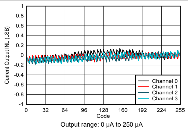
Figure 6-32. Current Output INL vs Digital Input Code
