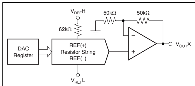
Figure 92. DAC8564 Architecture
