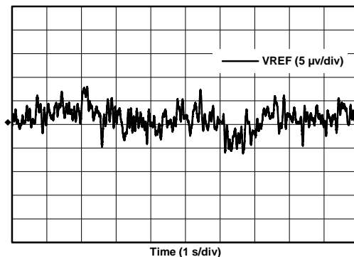
Figure 80. Internal Reference Noise, 0.1 Hz to 10 Hz
