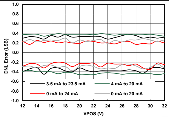
Figure 16. IOU Differential Linearity Error vs Power Supplies
