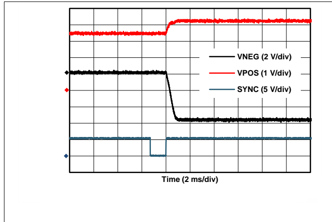
Figure 83. Buck-Boost Converter Power-On (IOUT Mode)
