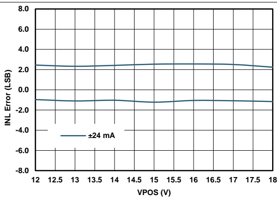
Figure 15. IOU Linearity Error vs Power Supplies
