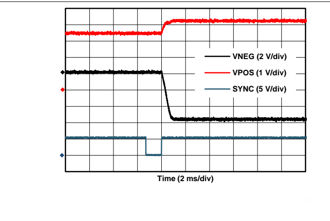
Figure 84. Buck-Boost Converter Power-On (VOUT Mode)
