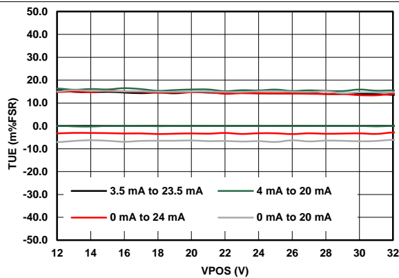
Figure 19. IOU Total Unadjusted Error vs Power Supplies
