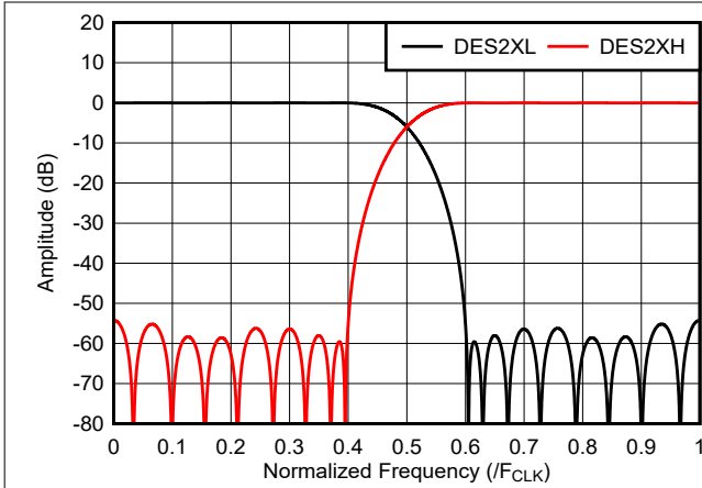
Figure 7-48. DES Interpolator Frequency Response
