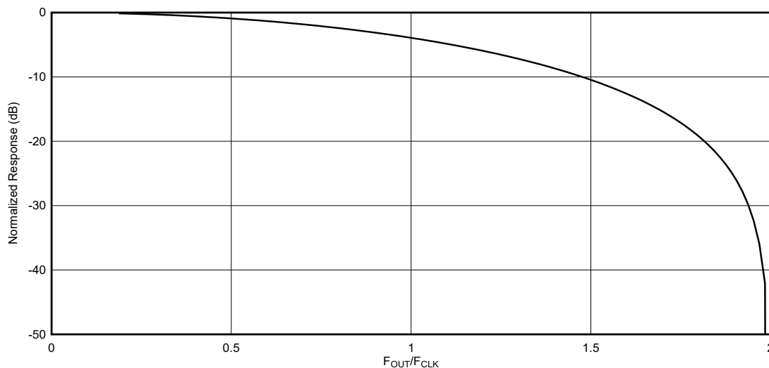
Figure 7-10. DES Output Frequency Response
