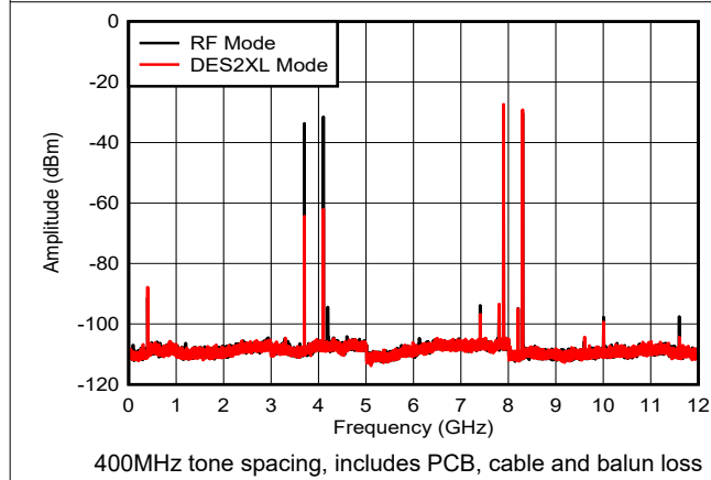
Figure 6-40. Dual Tone, f_{\text{OUT}} = 8097\text{MHz} , -12dBFS
