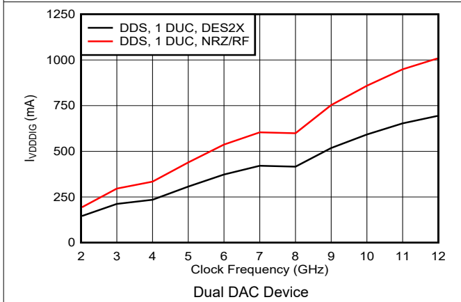
Figure 6-58. VDDDIG Current vs Clock Frequency and DAC Mode
