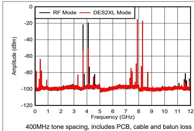
Figure 6-38. Dual Tone, f_{\text{OUT}} = 8097\text{MHz} , 0dBFS
