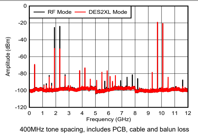
Figure 6-41. Dual Tone, f_{\text{OUT}} = 9897\text{MHz} , 0dBFS
