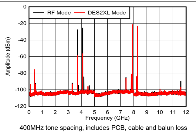
Figure 6-39. Dual Tone, f_{\text{OUT}} = 8097\text{MHz} , -6dBFS
