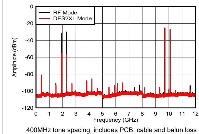
Figure 6-42. Dual Tone, f_{\text{OUT}} = 9897\text{MHz} , -6dBFS
