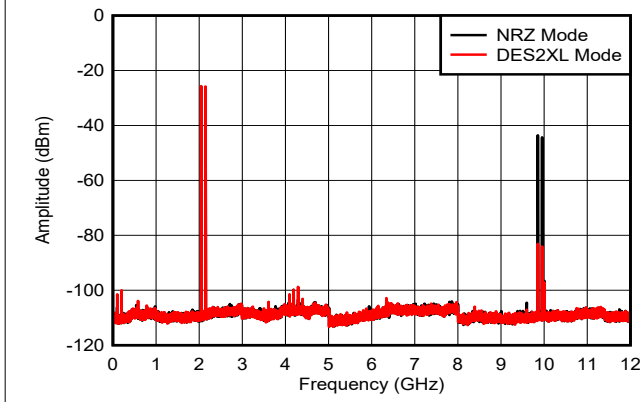
100MHz tone spacing, includes PCB, cable and balun loss
