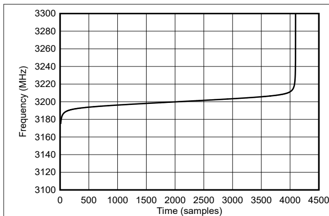
Figure 8-13. NLFM Frequency Ramp
