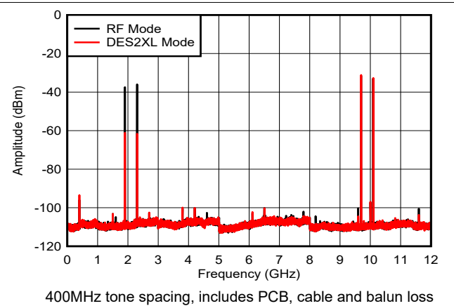
Figure 6-43. Dual Tone, f_{\text{OUT}} = 9897\text{MHz} , -12dBFS
