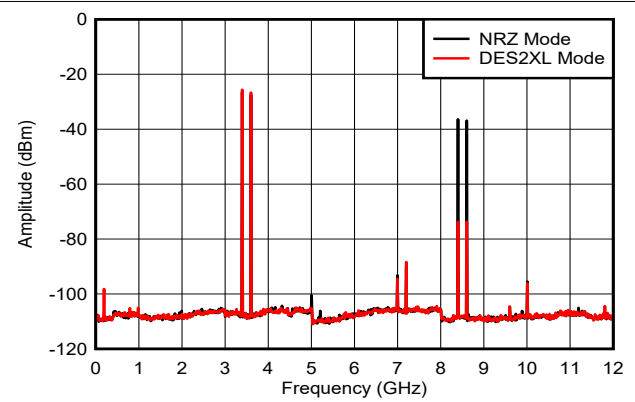
200MHz tone spacing, includes PCB, cable and balun loss
