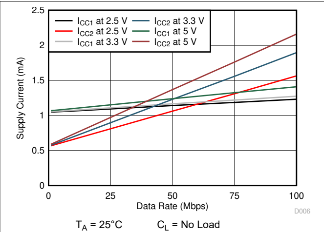
Figure 5-6. ISO7710 Supply Current vs Data Rate (With No Load)
