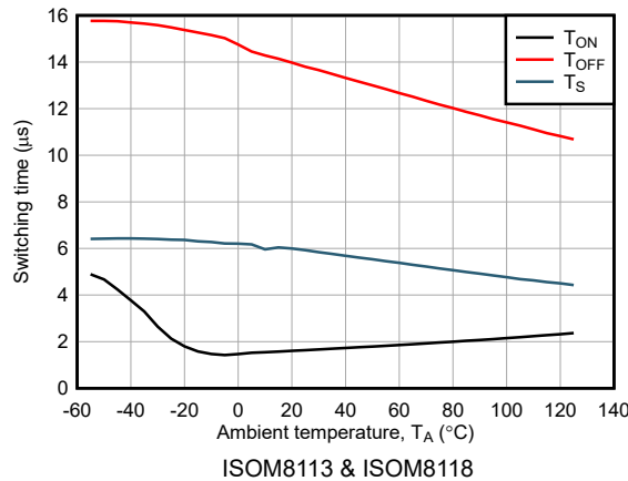
Figure 6-29. Switching Time vs Ambient Temperature
