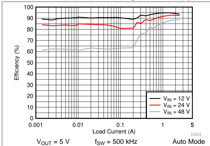
Figure 35. LM76002-Q1 Efficiency
