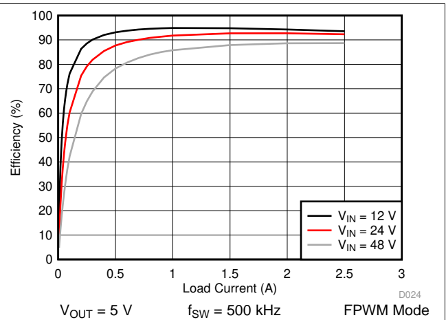
Figure 36. LM76002-Q1 Efficiency
