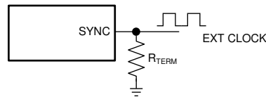
Figure 18. Frequency Synchronization
