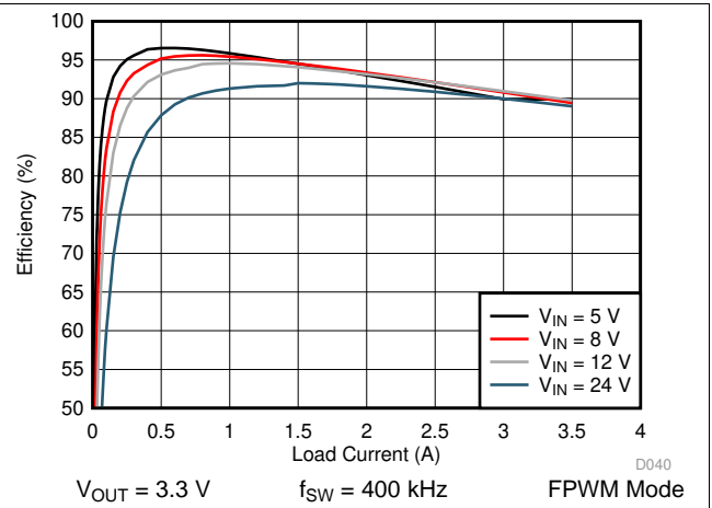
Figure 24. LM76003-Q1 Efficiency
