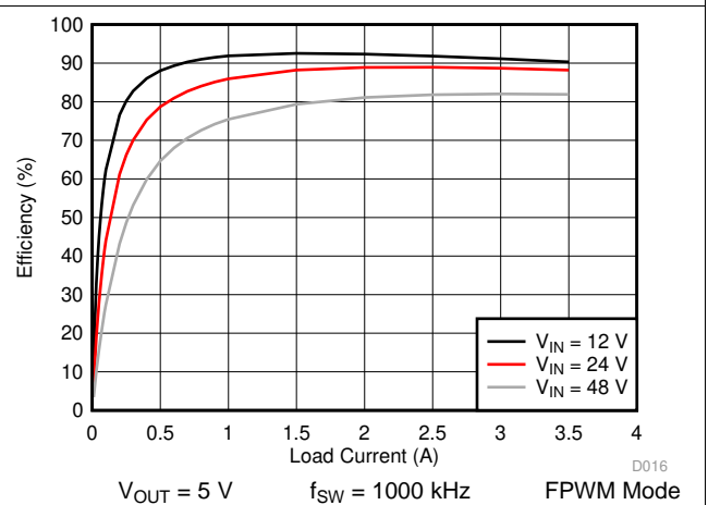
Figure 28. LM76003-Q1 Efficiency
