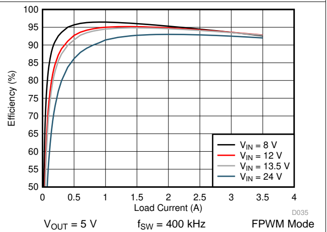
Figure 26. LM76003-Q1 Efficiency
