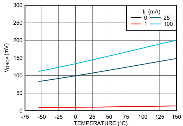
Dropout Voltage versus Temperature (New Chip)
