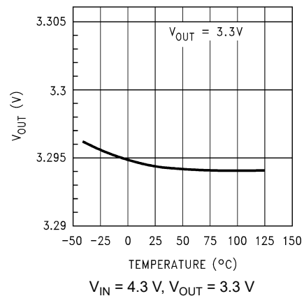
Figure 5-2. Output Voltage versus Temperature (Legacy Chip)
