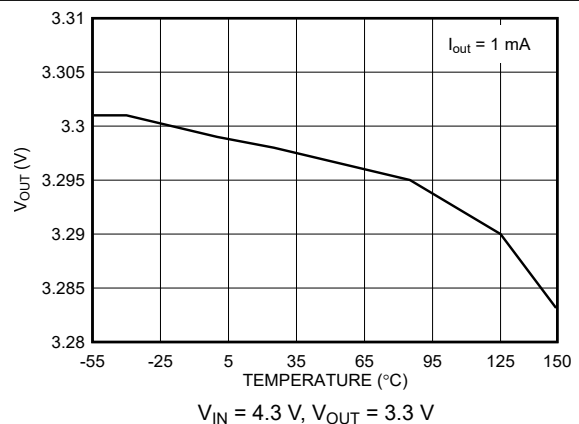
Figure 5-4. Output Voltage versus Temperature (New Chip)
