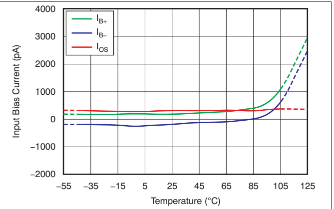
Figure 8. Input Bias Current vs Temperature
