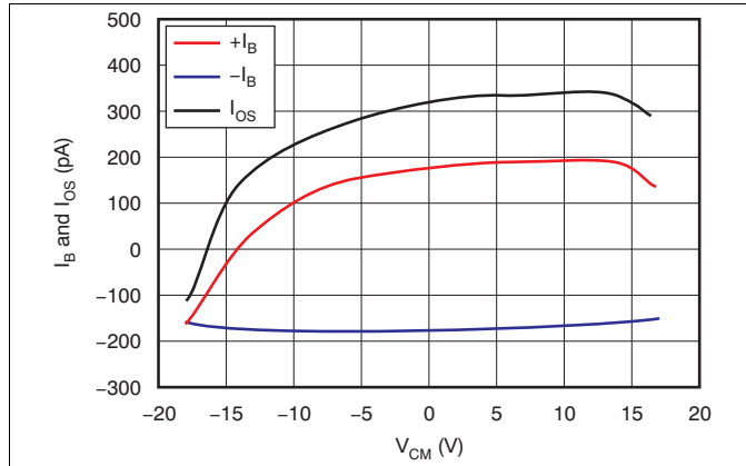
Figure 7. I_B and I_{OS} vs Common-Mode Voltage
