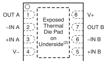
Figure 4-4. OPA2328 DRG Package, 8-Pin WSON (Top View)
