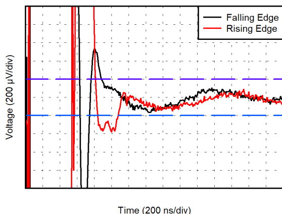
Figure 6-39. Settling Time
