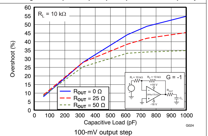
Figure 24. Small-Signal Overshoot vs Capacitive Load
