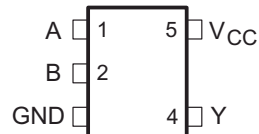
Figure 4-1. DBV Package 5-Pin SOT-23 Top View
