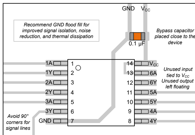
Figure 9-3. Example Layout for the SN74LV6T06-Q1
