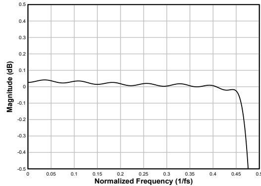
Figure 7-21. Linear Phase Decimation Filter Pass-Band Ripple
