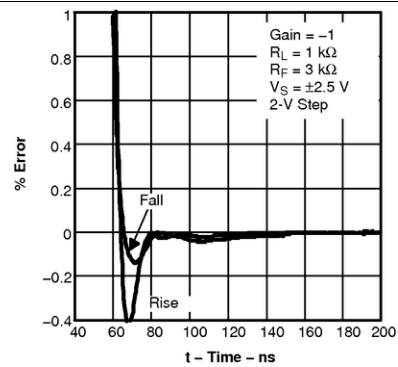
Figure 34. Settling Time
