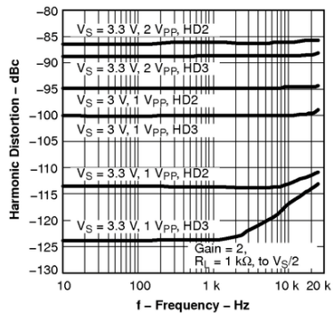
Figure 39. Harmonic Distortion vs Frequency
