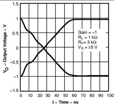
Figure 37. Settling Time
