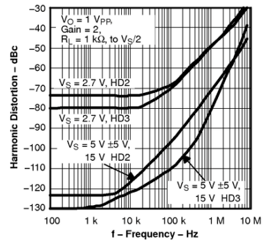
Figure 40. Harmonic Distortion vs Frequency
