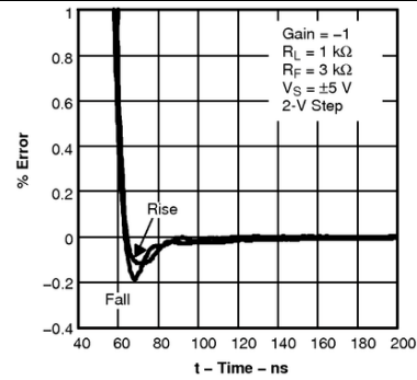
Figure 38. Settling Time
