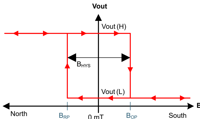
Figure 8-2. Latch Functionality
