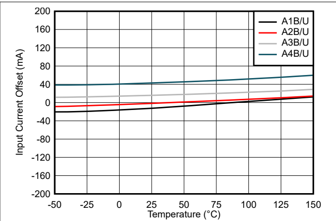
Figure 7-2. TMCS1108-Q1 Input Offset Current vs. Temperature
