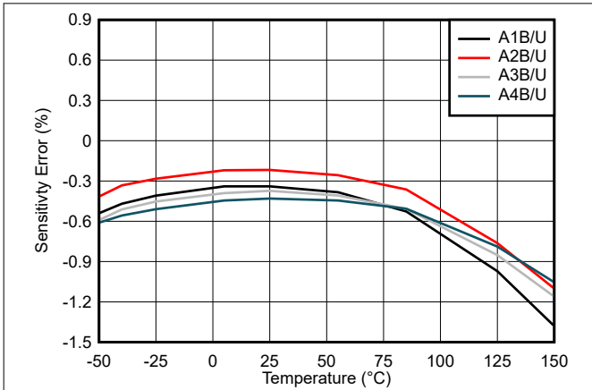
Figure 7-1. TMCS1108-Q1 Sensitivity Error vs. Temperature
