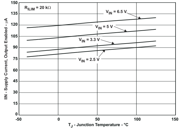
Figure 6-14. I_{IN} – Supply Current, Output Enabled – \mu\text{A}
