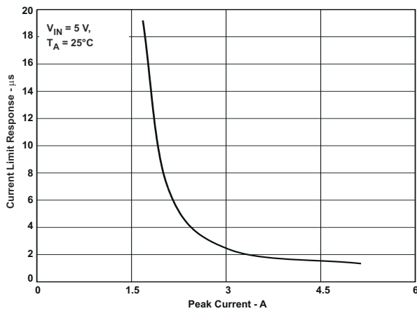
Figure 6-15. Current Limit Response – \mu\text{s}
