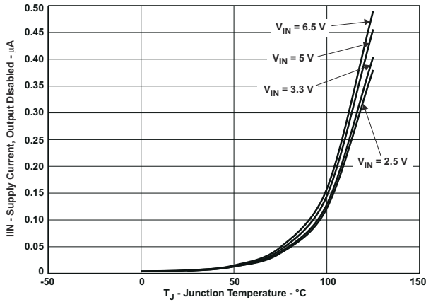
Figure 6-13. I_{IN} – Supply Current, Output Disabled – \mu\text{A}
