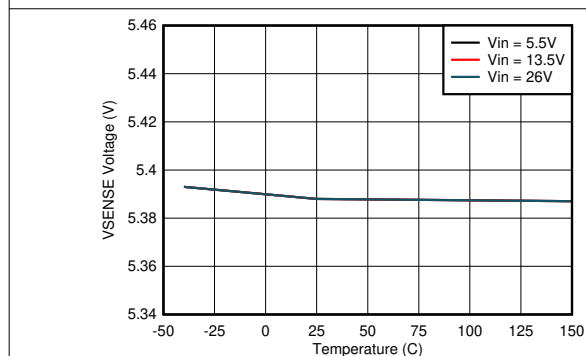
Figure 8-5. V_{SENSE} Voltage vs Junction Temperature
