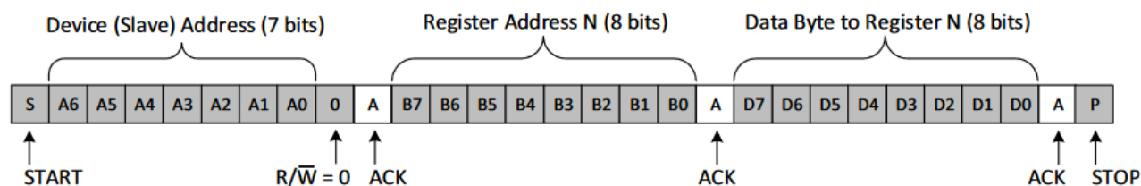
Figure 7-3. I 2 C write protocol
