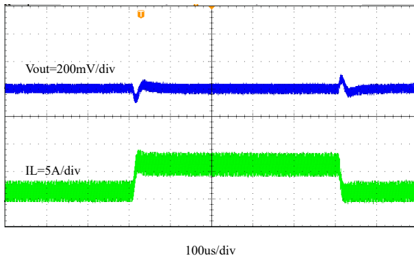
Figure 8-10. Transient Response, 1.6 A to 6.4 A with 2.5 A/us SR
