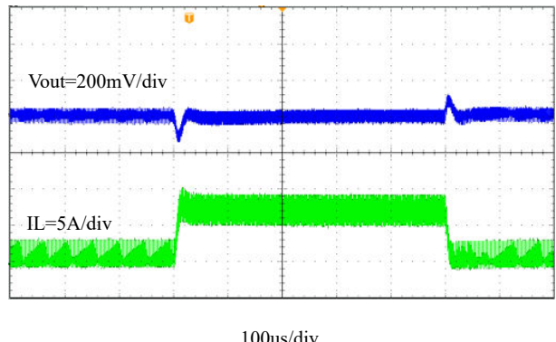
Figure 8-11. Transient Response, 0.8 A to 7.2 A with 2.5 A/us SR
