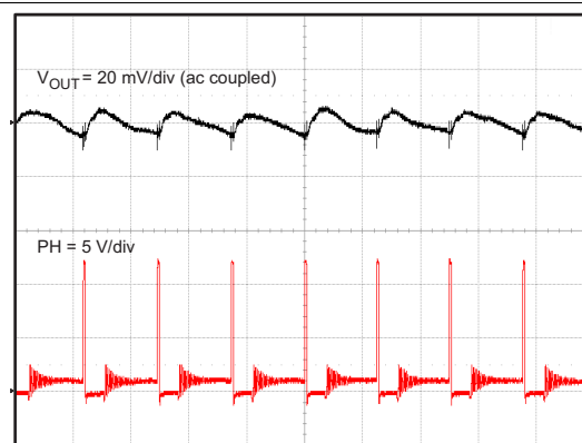
Time = 5 \mu s/div Figure 17. Output Ripple, I_{OUT} = 30 mA
