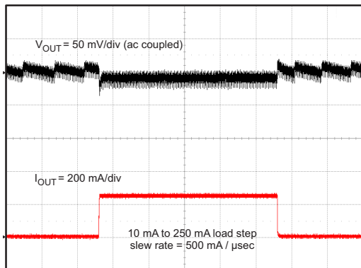
Time = 200 \mu s/div Figure 14. Transient Response, 2% to 50% Load Step
