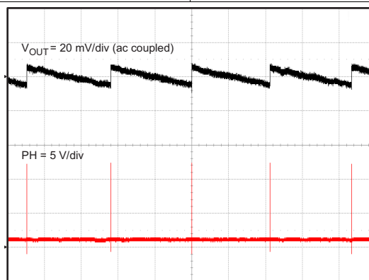
Time = 2 ms/div Figure 18. Output Ripple, I_{OUT} = 0 mA
