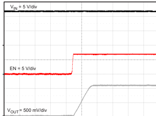
Time = 2 ms/div Figure 15. Start-Up Relative to EN
