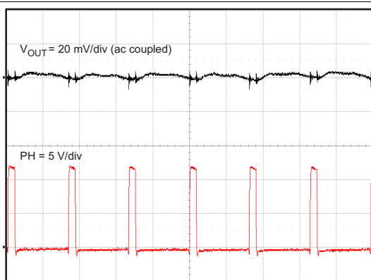
Time = 1 \mu s/div Figure 16. Output Ripple, I_{OUT} = 500 mA
