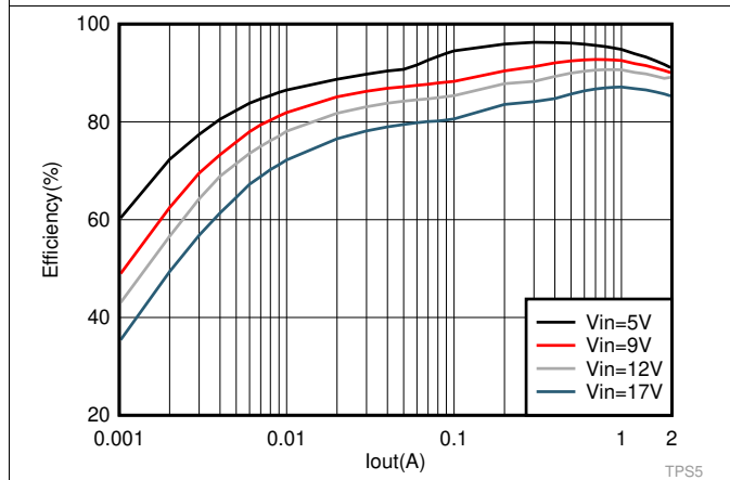
Figure 7. TPS562231 V OUT = 1.05 V Efficiency
