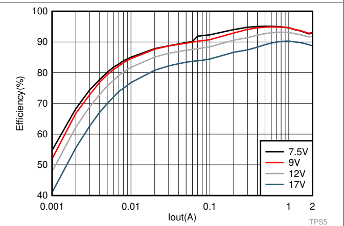
Figure 8. TPS562231 V OUT = 1.8 V Efficiency
