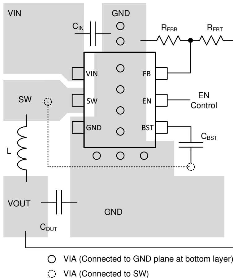
Figure 22. TPS562231 Layout
