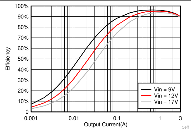
Figure 7-14. V_{OUT} = 5\text{-V} Efficiency, L = 4.7\ \mu\text{H}
