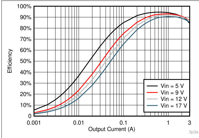
Figure 7-13. V_{OUT} = 3.3\text{-V} Efficiency, L = 3.3\ \mu\text{H}
