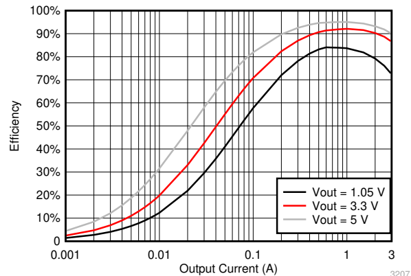
TPS563207S Efficiency
