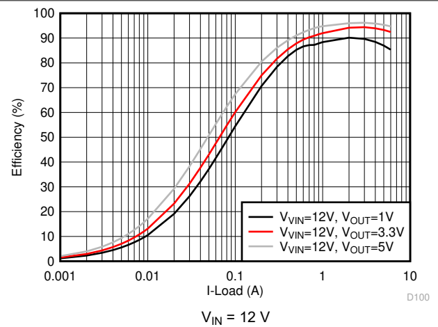
Figure 5-18. TPS566238 and TPS566238P Efficiency
